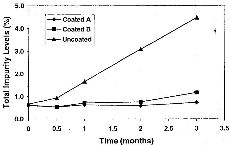
Graph A. Total Impurity Levels of Budesonide (0.22%) in Solution Formulations (HFA-134a/Ethanol 11%) in Three Different Containers, Incubated at 40°C/75%RH
