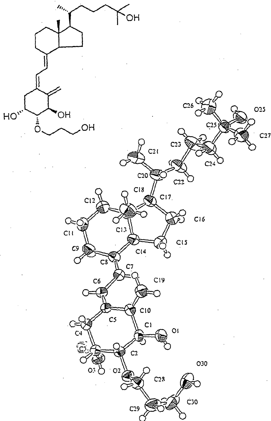
Structure of ED-71 (1)
