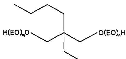
[Chemical formula 17]
