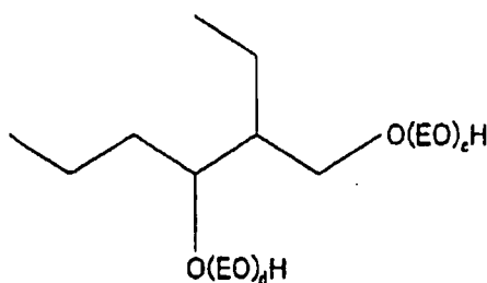
[chemical formula 7]
