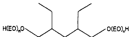
[Chemical formula 14]
