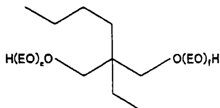
[chemical formula 8]
