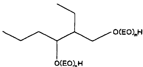
[Chemical formula 15]
