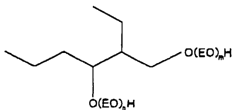
[Chemical formula 16]
