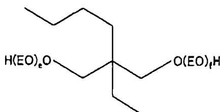
[chemical formula 17]
