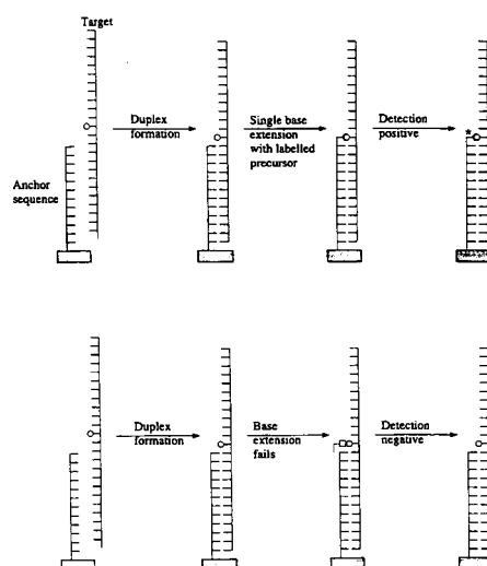
Detection of point mutation by single base extension
