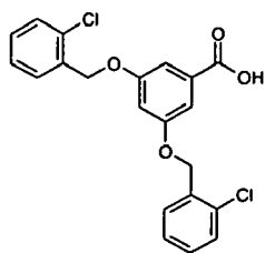
Compound (b)
