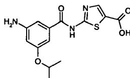
Compound (k)
