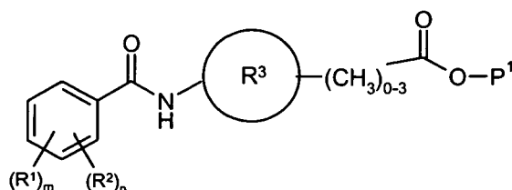
Formula (IIIc)
