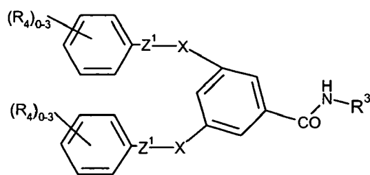
Formula (II)
