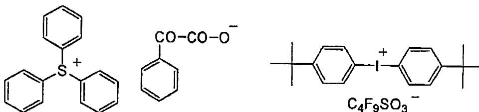
Polymerization initiator (1)
