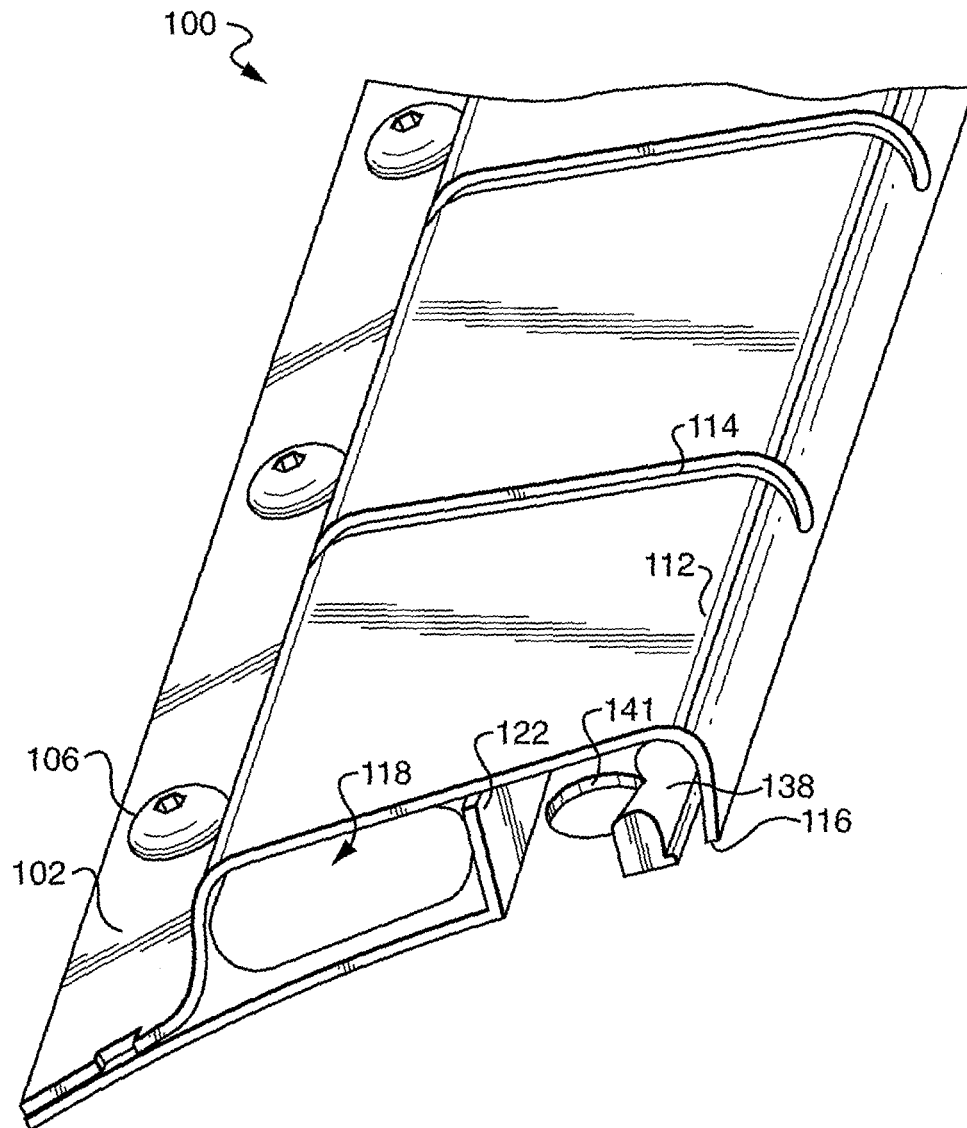
FIG. 6 (PRIOR ART)
