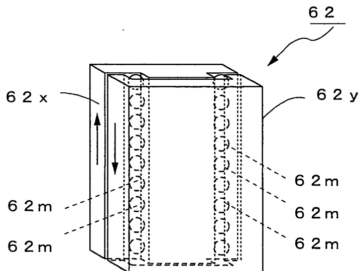
FIG.8 PRIOR ART
