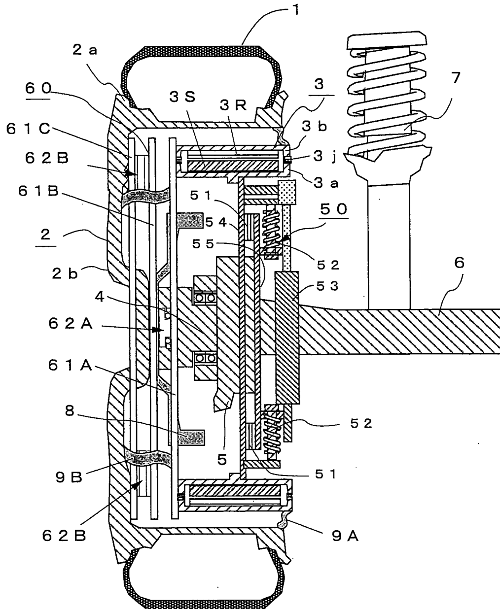
FIG.6 PRIOR ART
