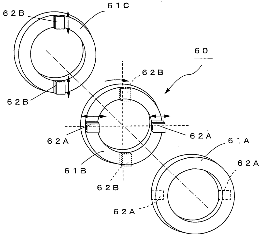
FIG.8 PRIOR ART
