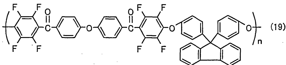
[Chemical Formula 13]
