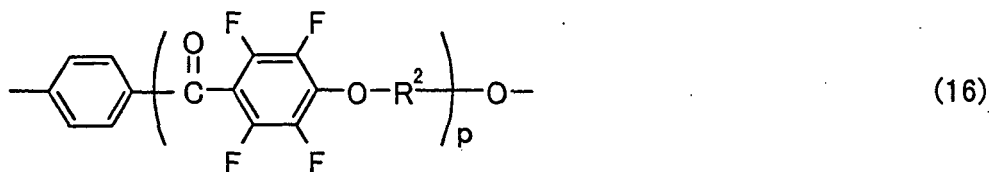
[Chemical Formula 10]
