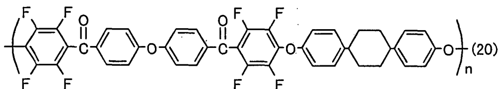
[Chemical Formula 14]
