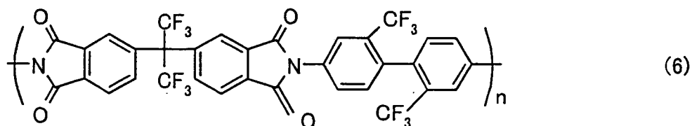
[Chemical Formula 6]
