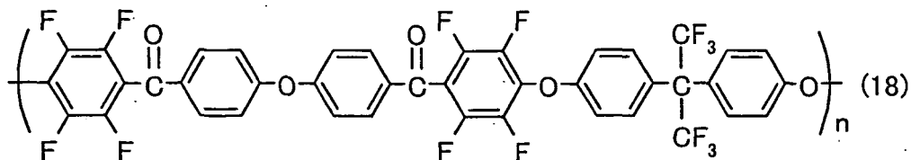
[Chemical Formula 12]
