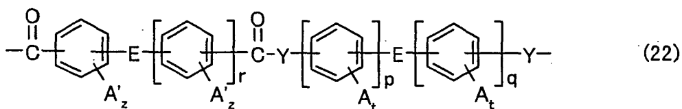
[Chemical Formula 16]
