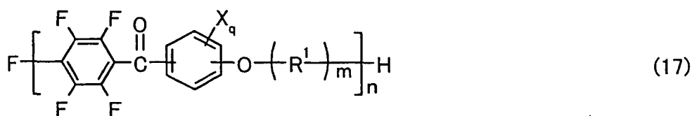
[Chemical Formula 11]
