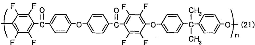
[Chemical Formula 15]
