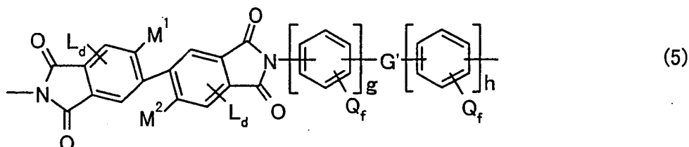
[Chemical Formula 5]
