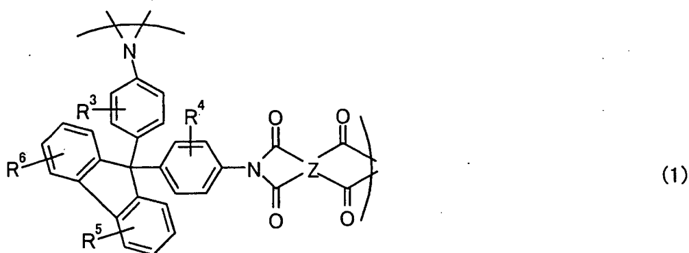
[Chemical Formula 1]
