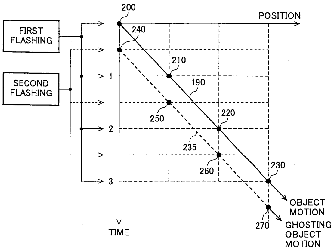
GHOSTING IMAGE FROM DOUBLE FLASHING
