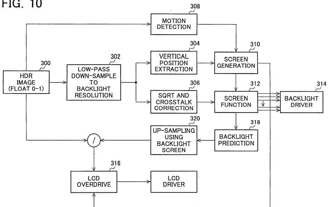
CONVERSION FROM HDR IMAGE TO BACKLIGHT AND LCD MODULATOR
