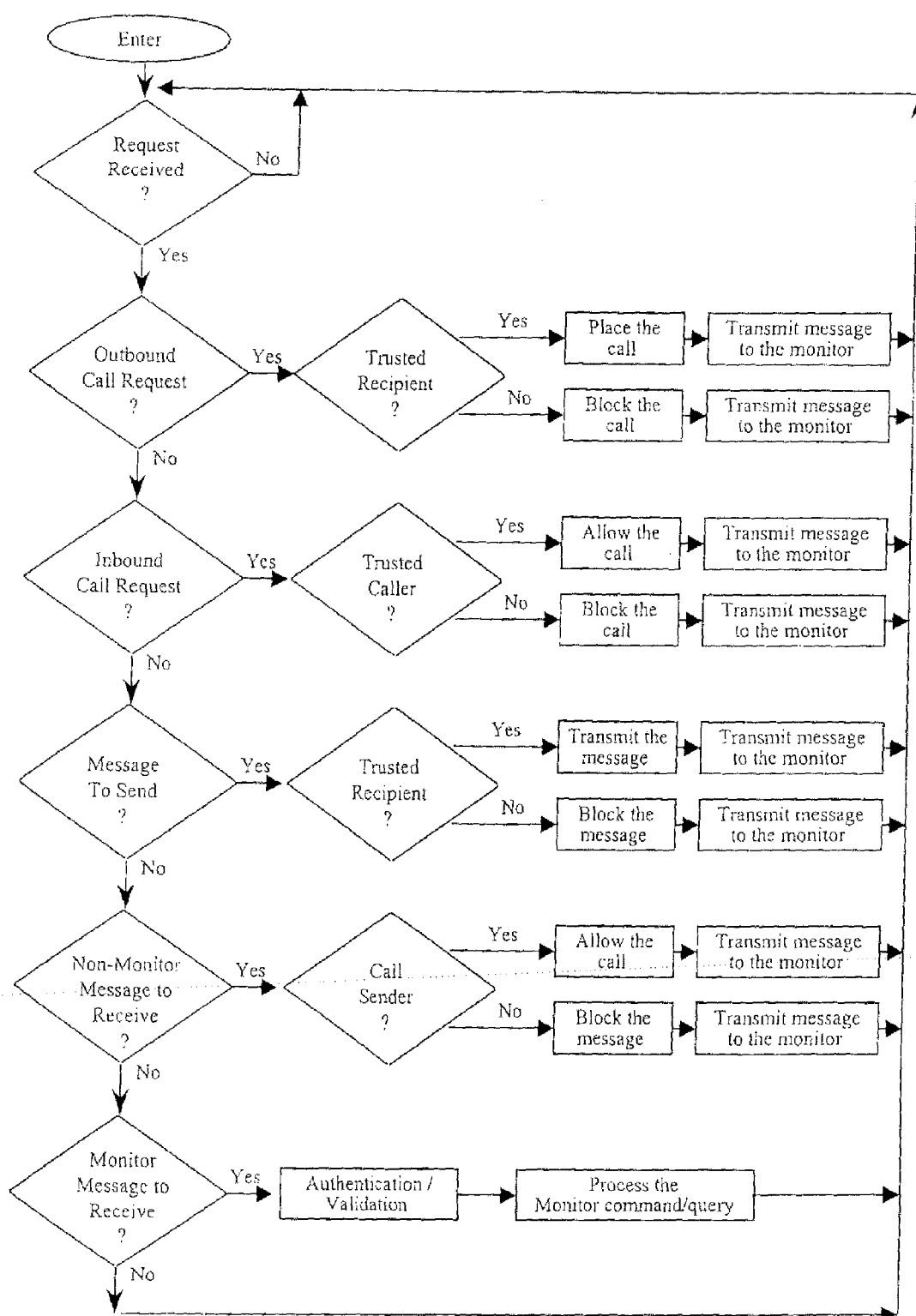
Figure 2 –Flow Logic
