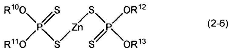
[Chemical Formula 16]
