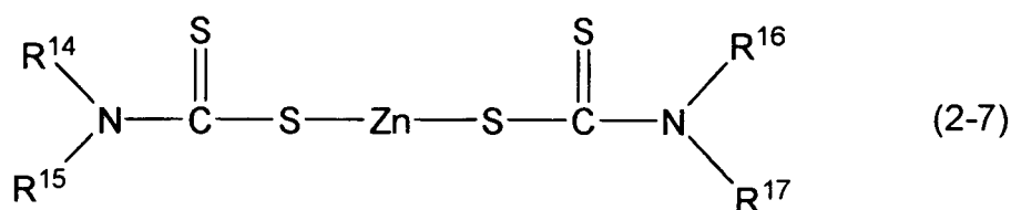
[Chemical Formula 18]
