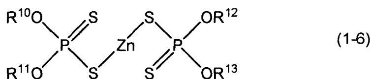
[Chemical Formula 3]
