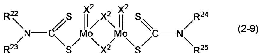
[Chemical Formula 19]
