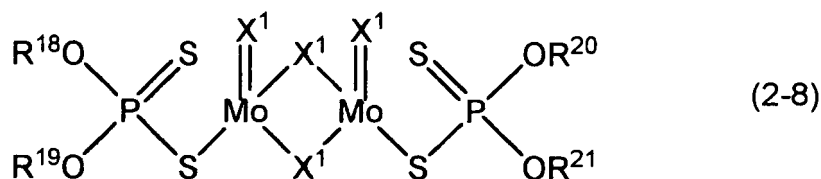
[Chemical Formula 18]
