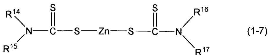
[Chemical Formula 5]
