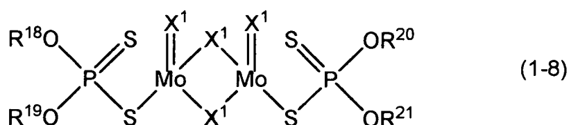
[Chemical Formula 5]
