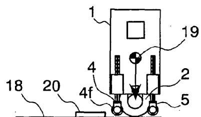
INVERTED TWO-WHEELS TRAVEL CONDITION
