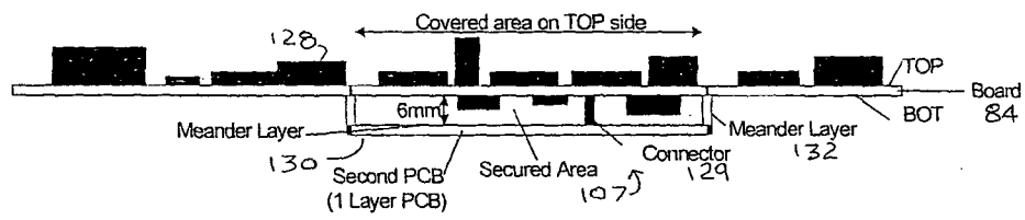
Close Up of Secure Area on Board
