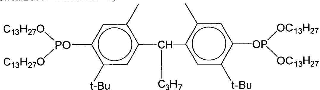
[Chemical formula 4]
