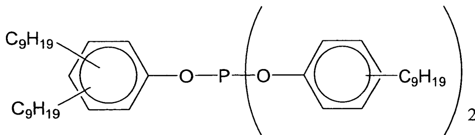
[Chemical formula 2]
