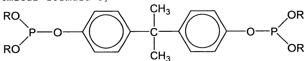
[Chemical formula 3]
