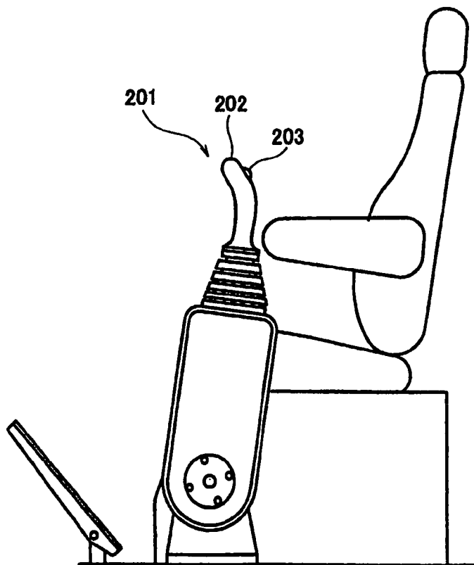
FIG. 9 PRIOR ART
