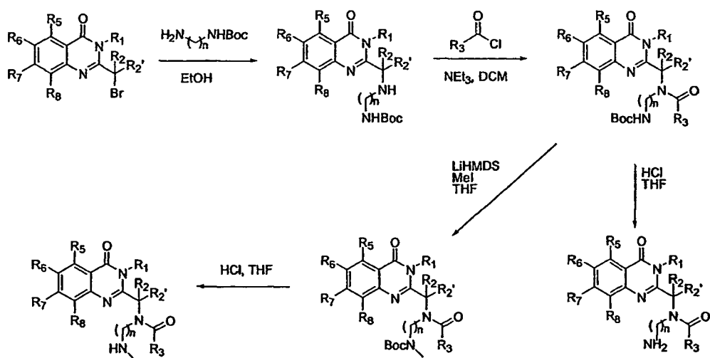
Figure 5d: Primary and Secondary Amine R_4 Synthesis
