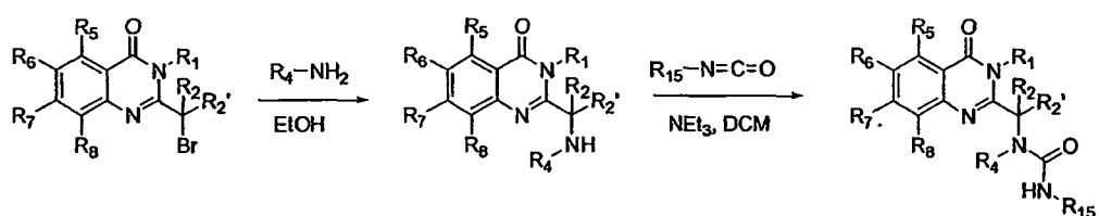
Figure 5d: Primary and Secondary Amine R_4 Synthesis
