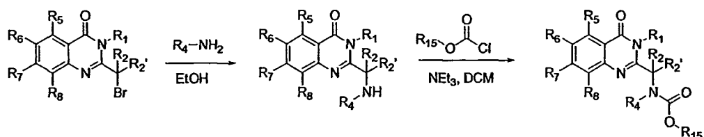
Figure 5c: Urea Synthesis
