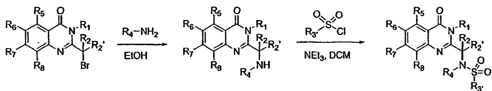
Figure 5a: Sulfonamide Synthesis
