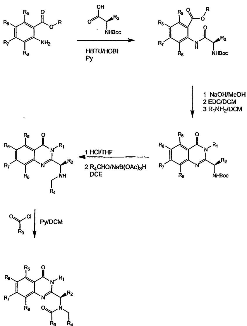
Figure 4: Asymmetric Synthesis
