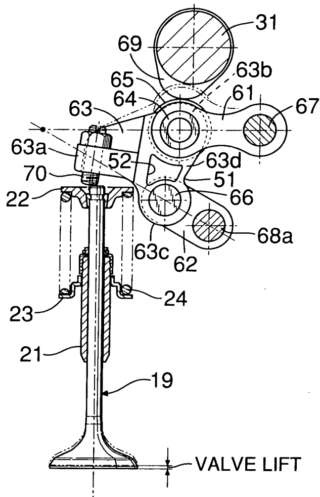
FIG.8B LOW VALVE LIFT
