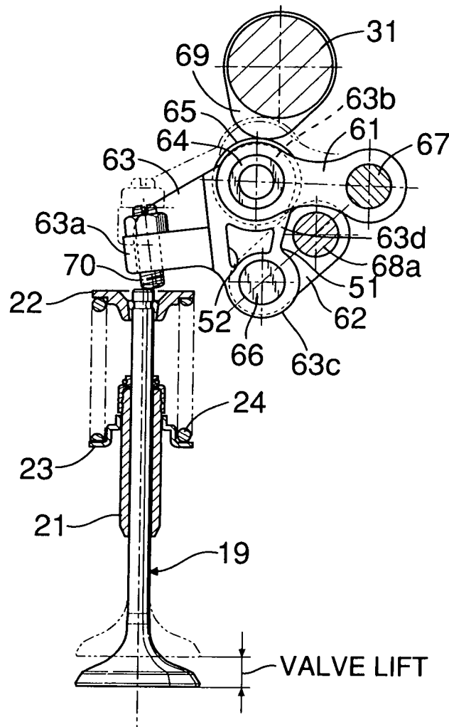
FIG.8A HIGH VALVE LIFT
