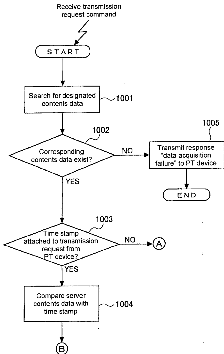
Flowchart part 1 showing PC server operation
