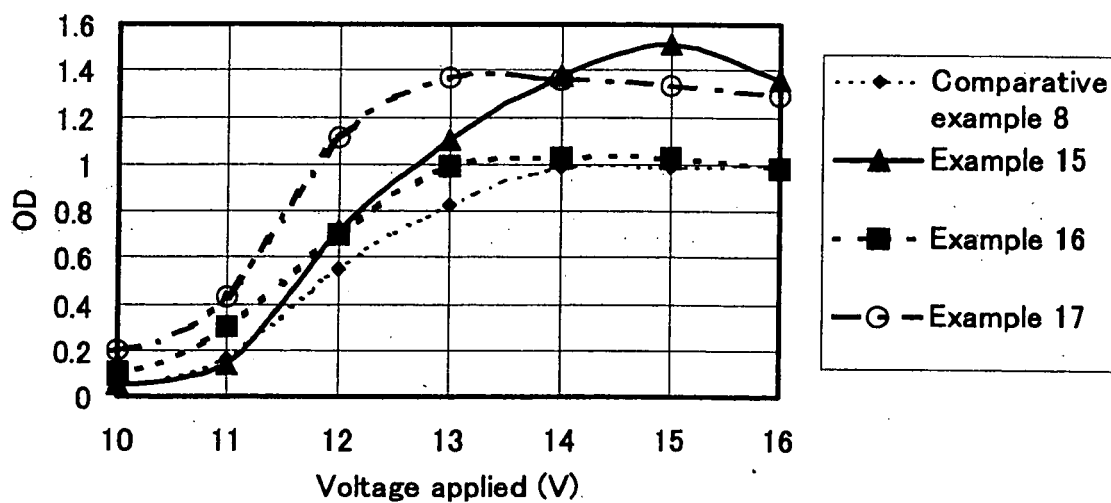
Dynamic Sensitivity characteristic curve
