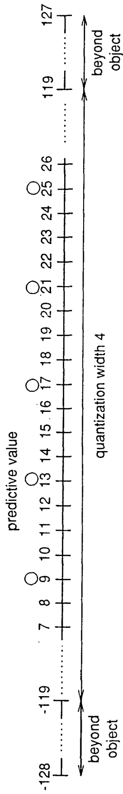
Fig.32 (a) linear quantization representative value
