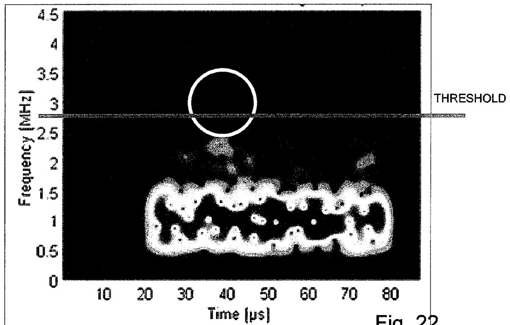
Graphic representation of Gabor expansion of RF signal
