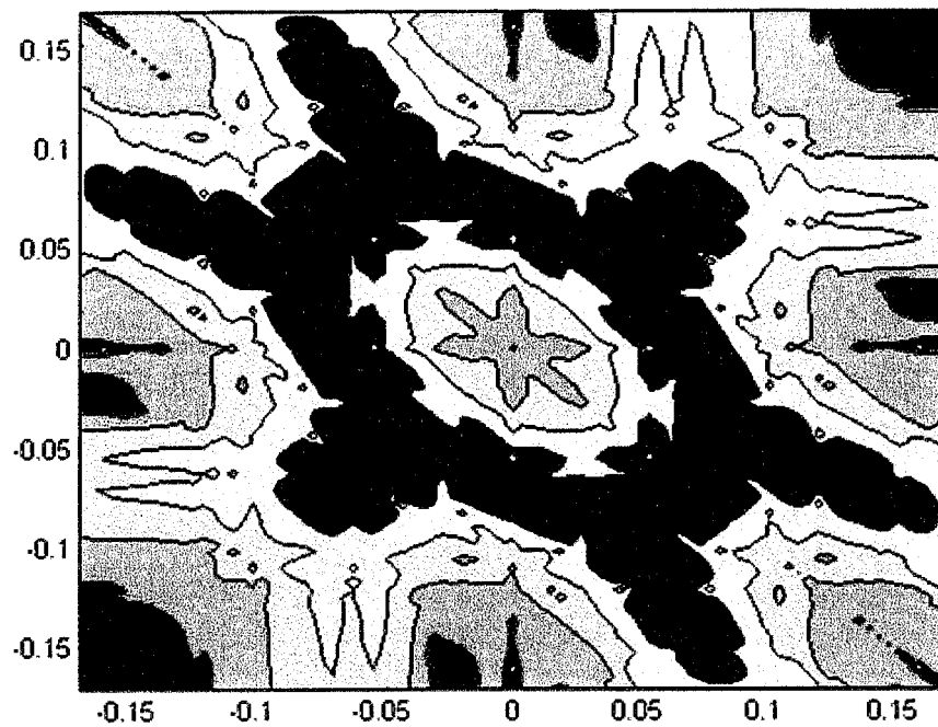
Bispectrum for simple tissue
