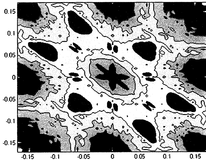
Bispectrum for tissue + bubble
