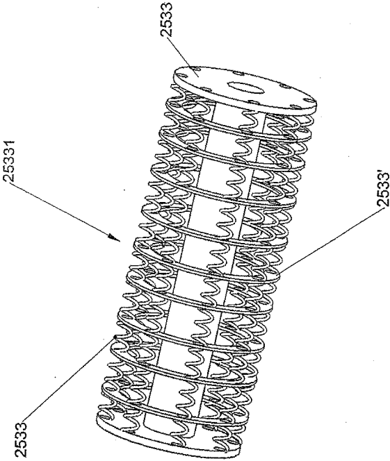
FIG 6C
