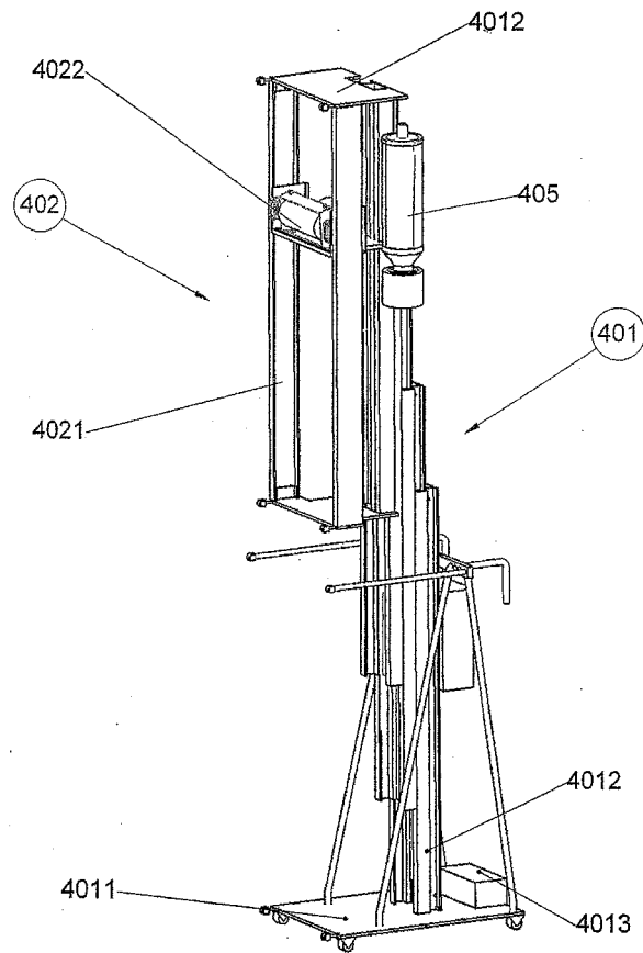
FIG 1C
