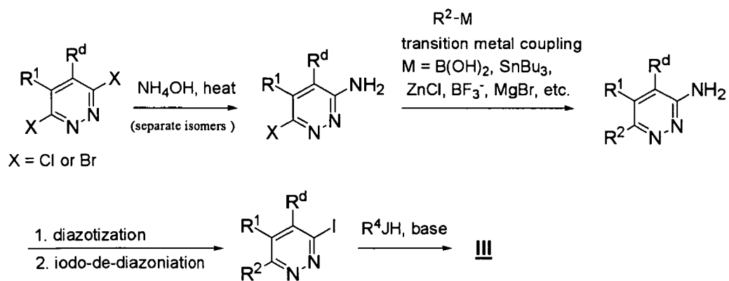
Scheme 3.d
