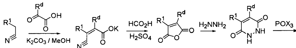
Scheme 3.c
