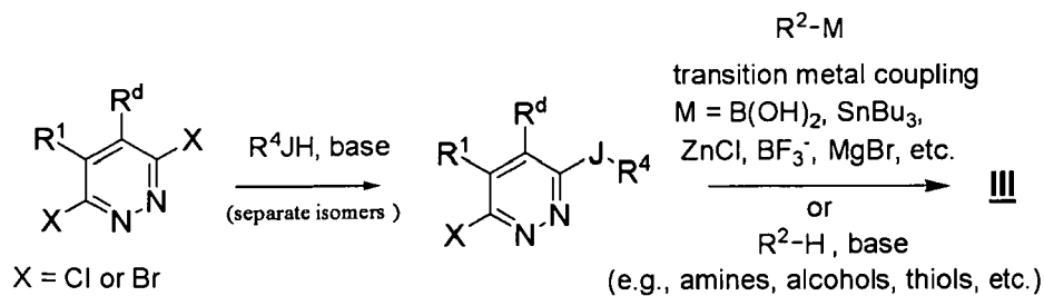
Scheme 3.c
