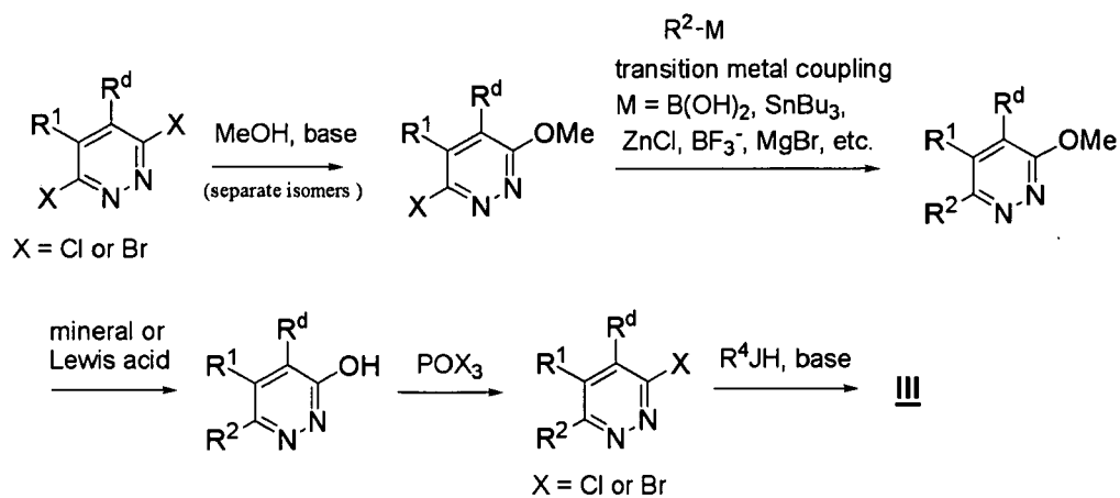
Scheme 3.d
