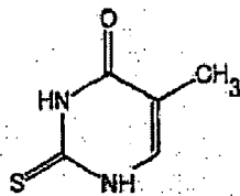
5-Methyl-2-thiouracil
