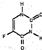
5-Fluorouracil
