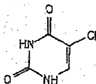
5-Chlorouracil
