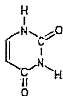
6-methyluracil
