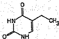
5-Ethyluracil
