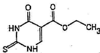
Ethyl 2-thiouracil-5-carboxylate
