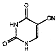
5-Cyanouracil
