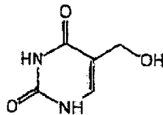
5-(Hydroxymethyl)uracil
