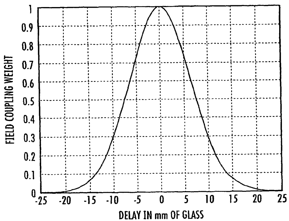
IMPULSE RESPONSE OF 10 GHz BANDPASS GAUSSIAN FILTER
