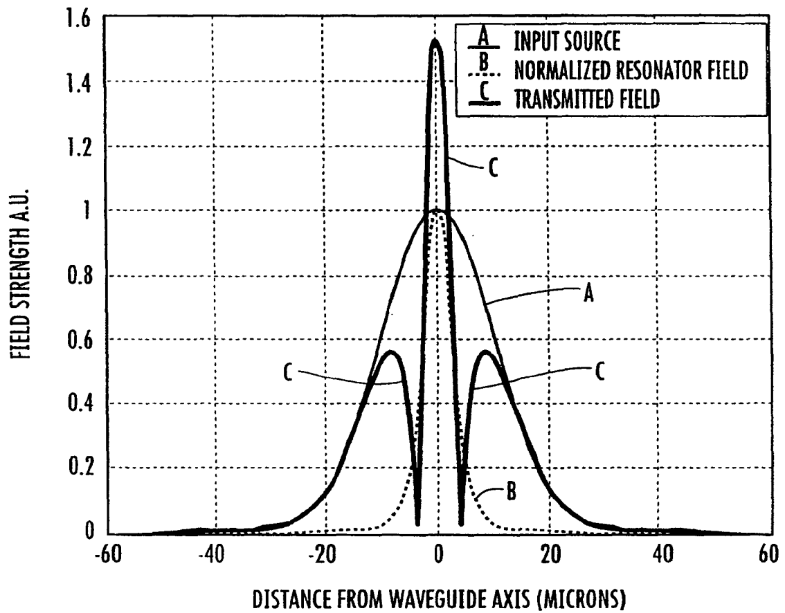
STEADY STATE FIELD PATTERNS
