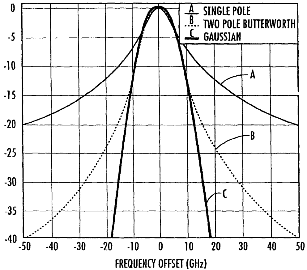
BANDSHAPE FOR GAUSSIAN AND BUTTERWORTH FILTERS
