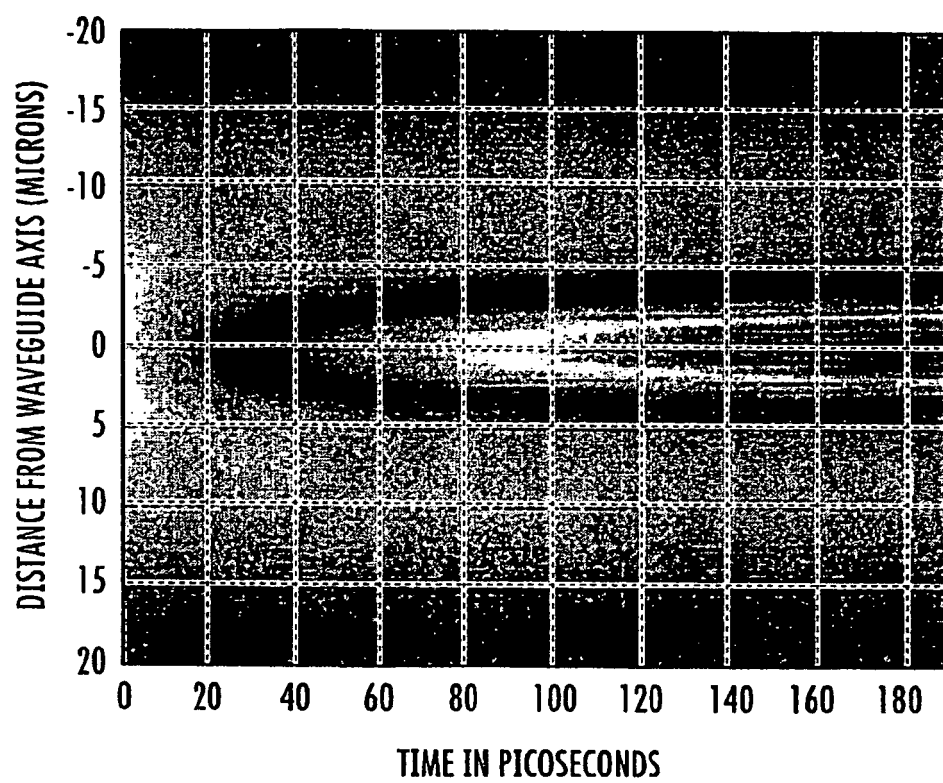
TRANSIENT FIELD PATTERNS IN SOURCE GUIDE
