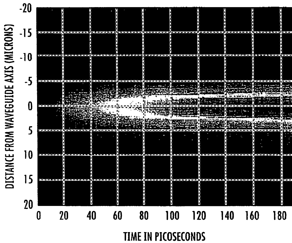
TRANSIENT FIELD PATTERNS IN RESONATOR GUIDE
