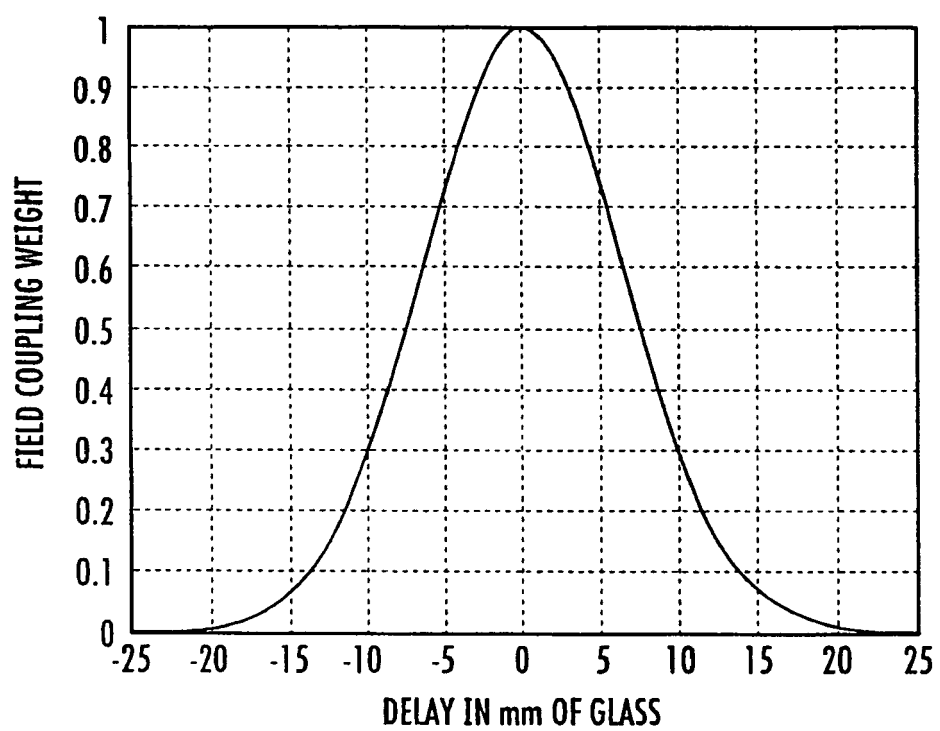
IMPULSE RESPONSE OF 10 GHz BANDPASS GAUSSIAN FILTER
