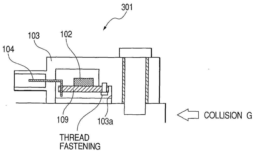
FIG. 18 COMPARATIVE ARRANGEMENT
