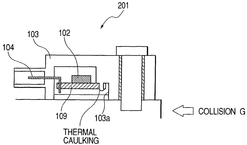
FIG. 17 COMPARATIVE ARRANGEMENT
