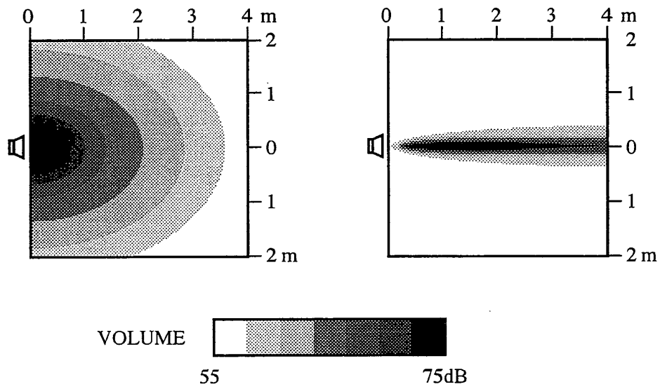
(a) NONDIRECTIONAL SPEAKER (b) ULTRA-DIRECTIONAL SPEAKER
