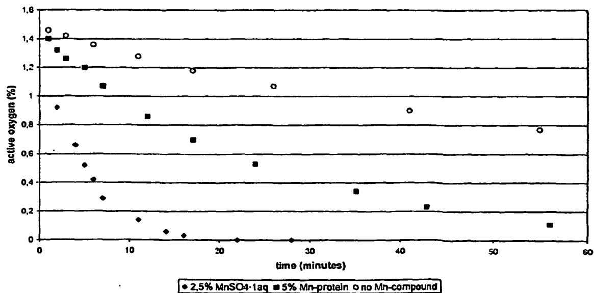
Decrease of active oxygen content in a 1% detergent solution in water (60°C, 6°GH) detergent contains various amount of Manganese compounds
