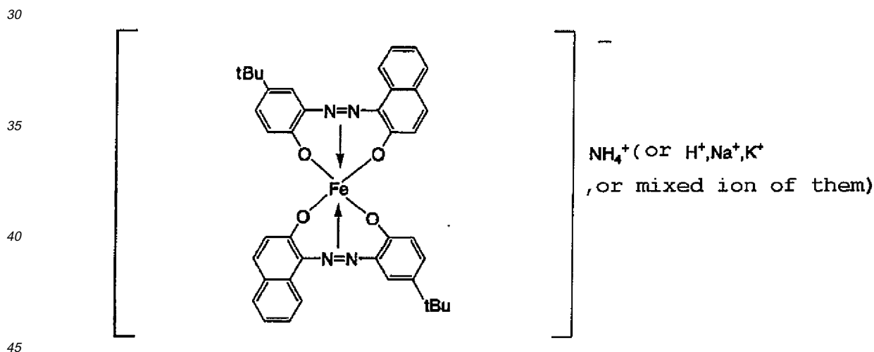
Azo-based iron complex compound (13)
