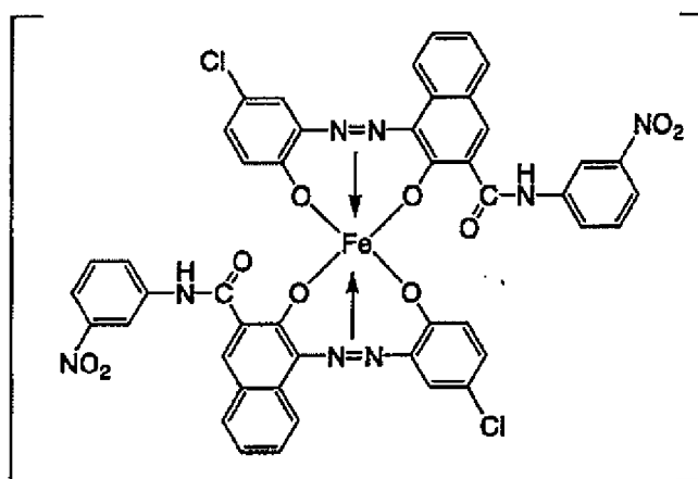
[0162] Azo-based iron complex compound (4)
