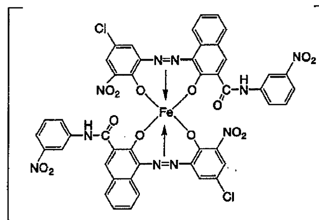
[0163] Azo-based iron complex compound (5)
