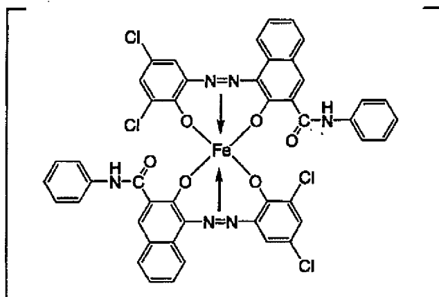
[0161] Azo-based iron complex compound (3)
