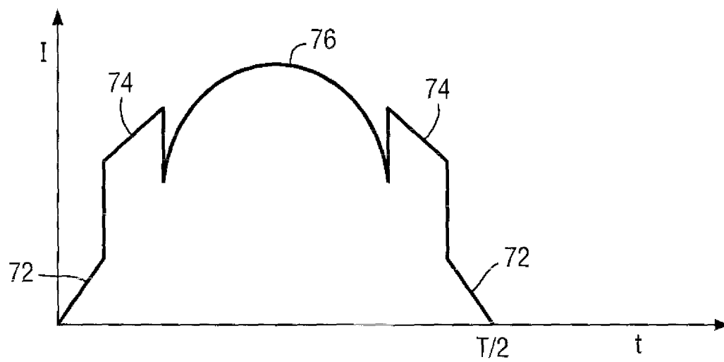
Fig.4. (Prior Art)
