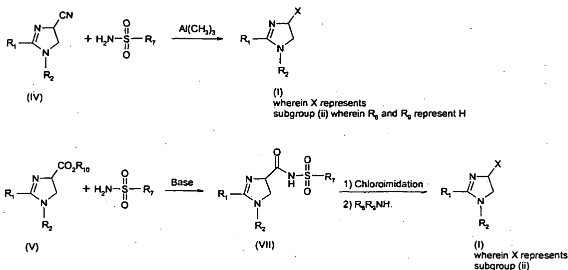
Scheme 2
