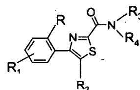
thiazoles
