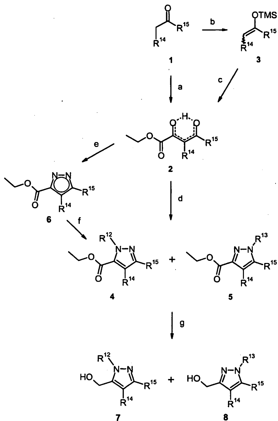
Scheme 3
