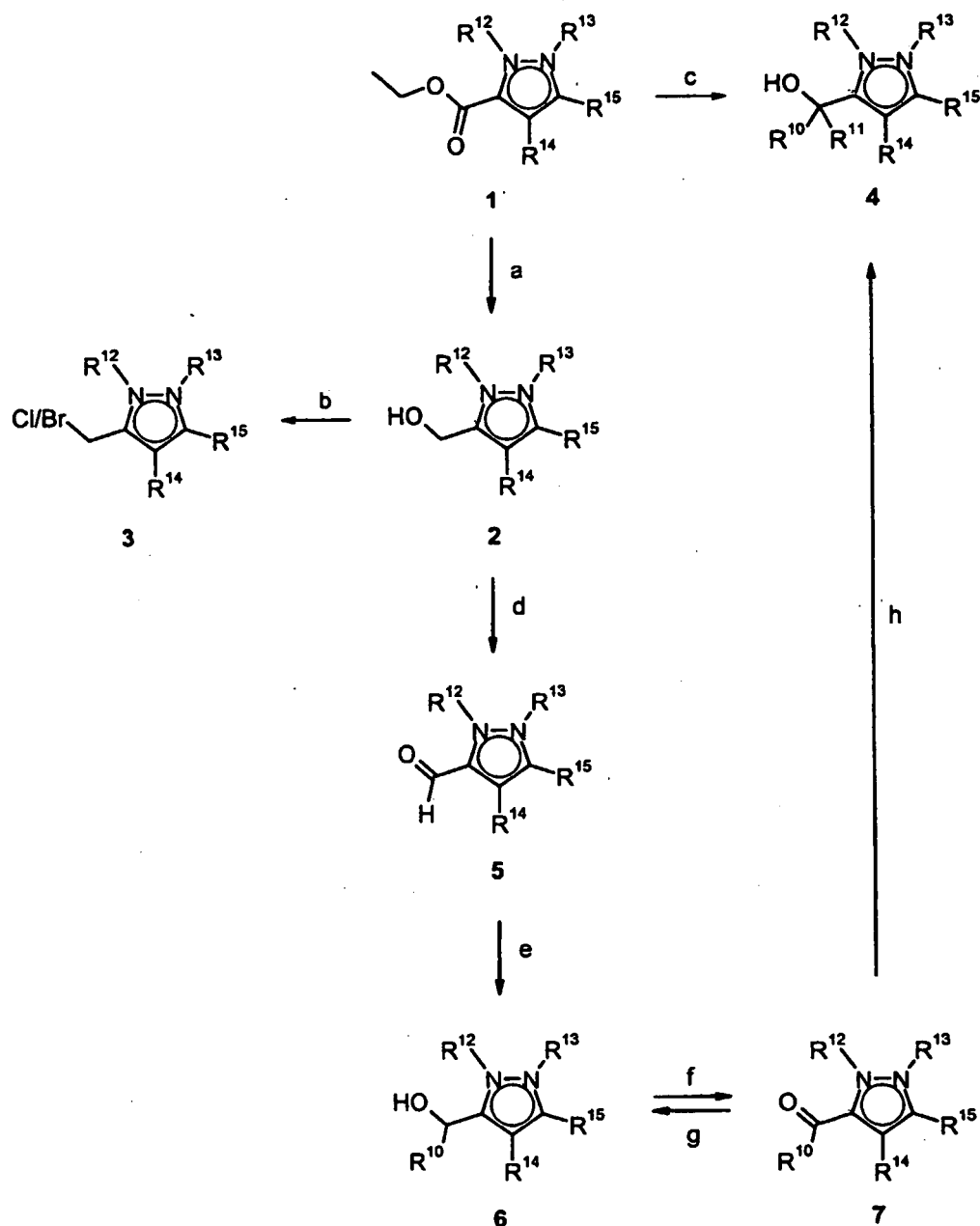
Scheme 4
