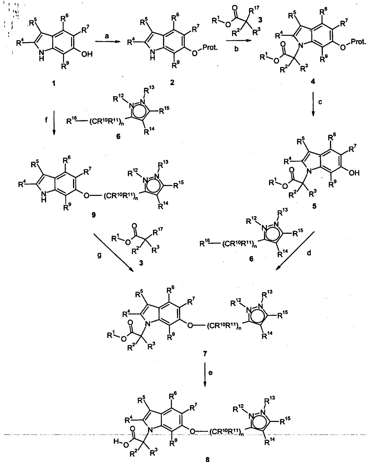
Scheme 1
