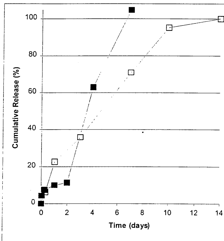
Fig 2. In vitro - in vivo correlation for the microcapsules prepared in Example 4. The in vivo release (open squares) was calculated from the plasma levels assuming 100% bioavailability and the in vitro release (closed squares) was determined according to Reslow et al (supra) with the exception that only 40 mg of microcapsules were used and no \alpha -amylase was added.
