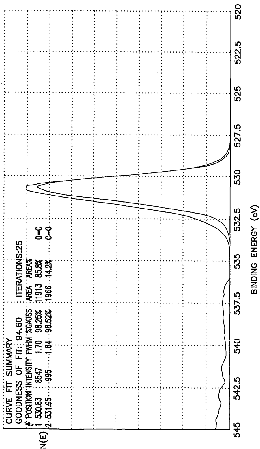
FIG. 5 ESCA O1s SPECTRA FOR HEAT-TREATED SAMPLE 6A
