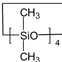
(X) octamethyl cyclotetrasiloxane
