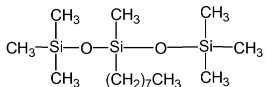
Chemical Formula (i)
