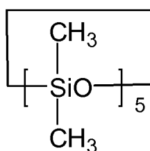
(IX) decamethyl cyclopentasiloxane
