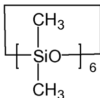
(VIII) dodecamethyl cyclohexasiloxan
