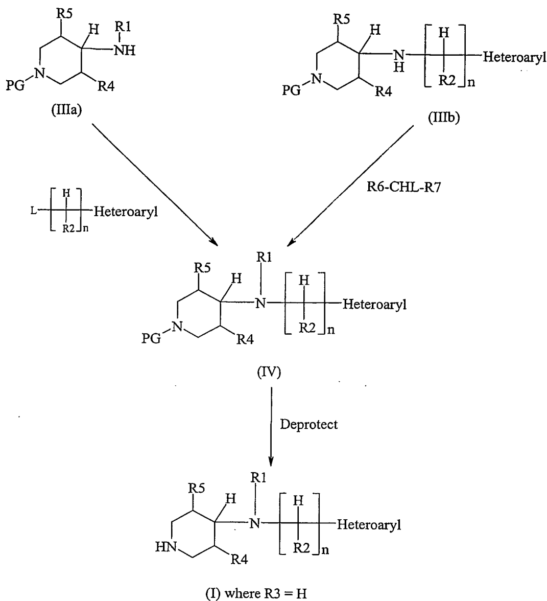
Scheme 2
