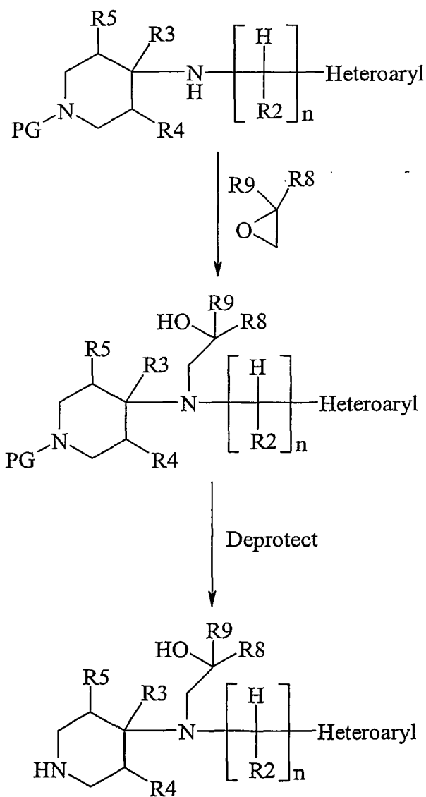
Scheme 3
