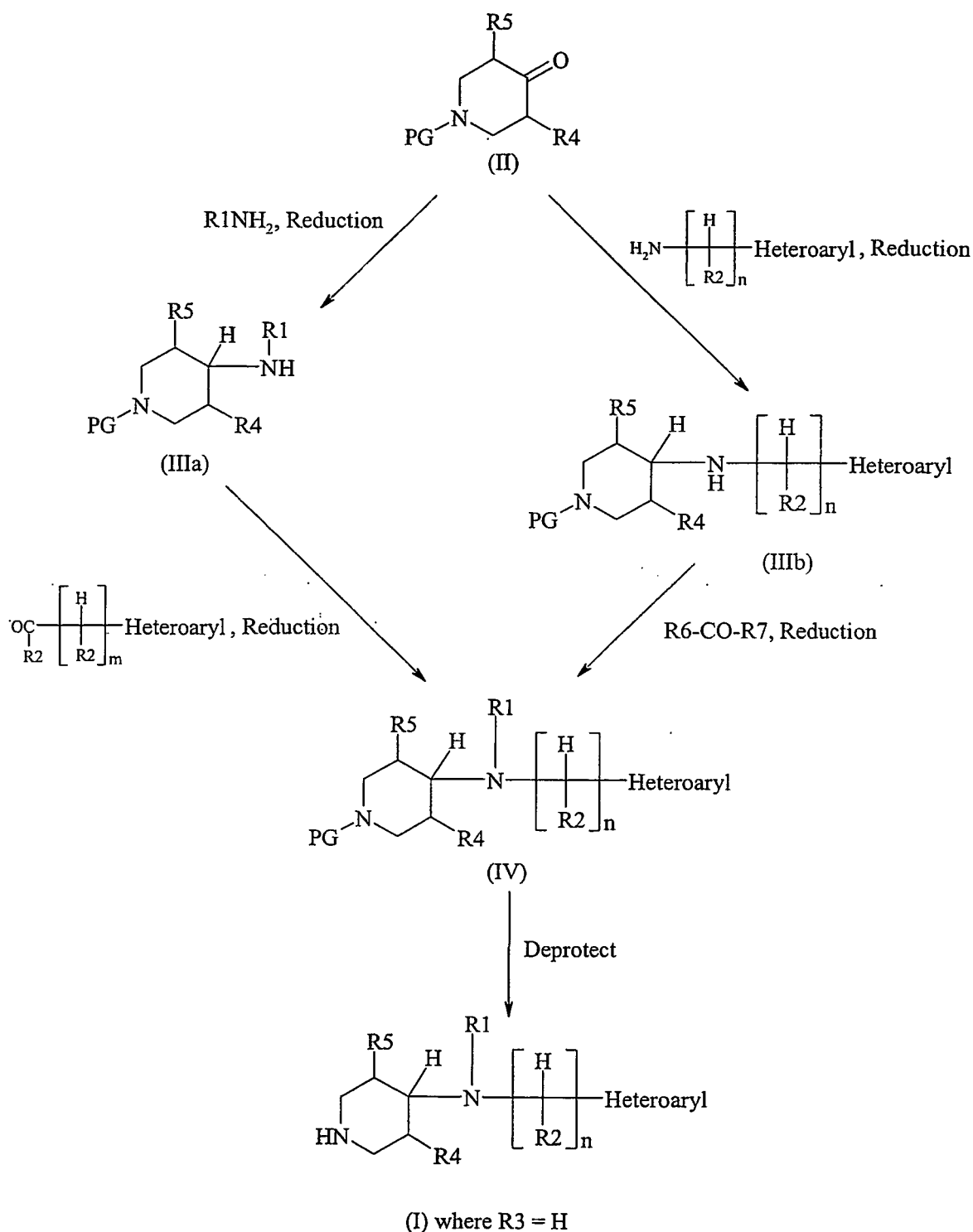
Scheme 1
