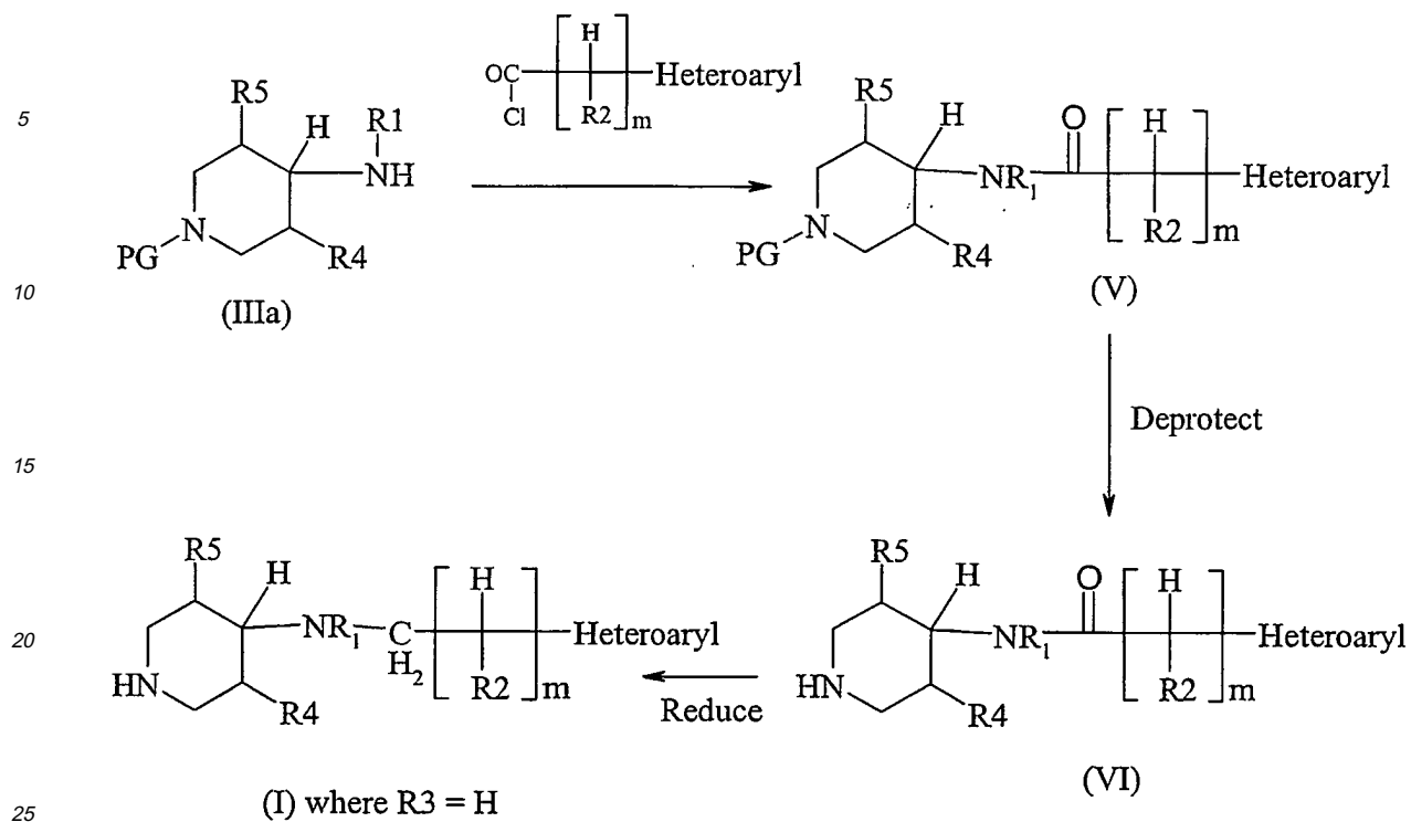
Scheme 4
