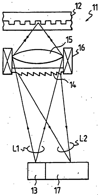
FIG. 1 PRIOR ART
