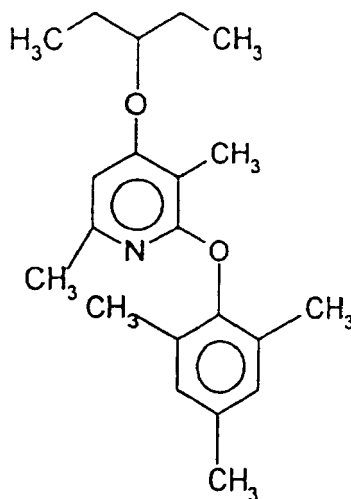
Compound 2
