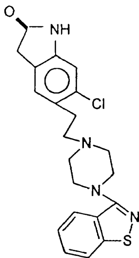
Compound 3
