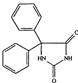
Compound 6
