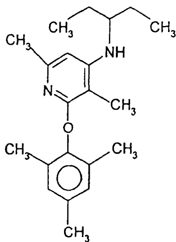
Compound 8
