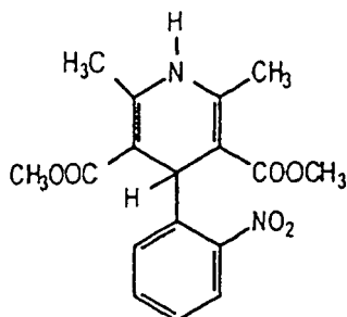
Compound 5
