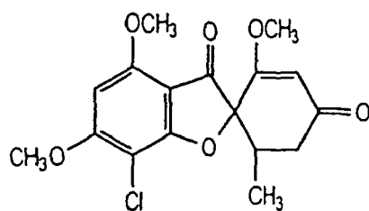
Compound 4
