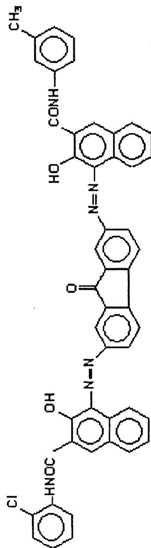
Chemical structure 1
