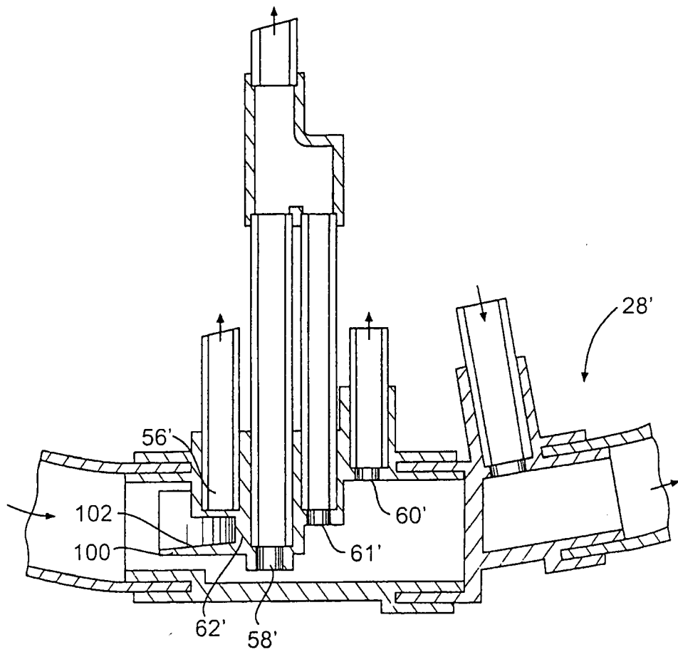
FIG. 3 (PRIOR ART)
