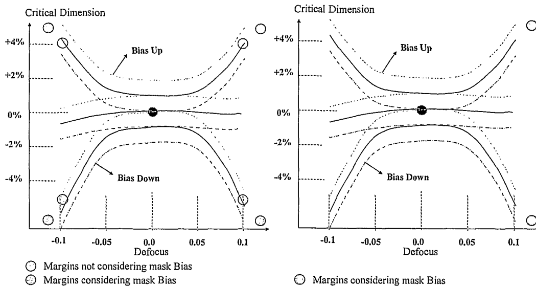
Figure 26. Dose, Defocus and Mask Bias variations and their impact in CD for a clear field, dark feature.
