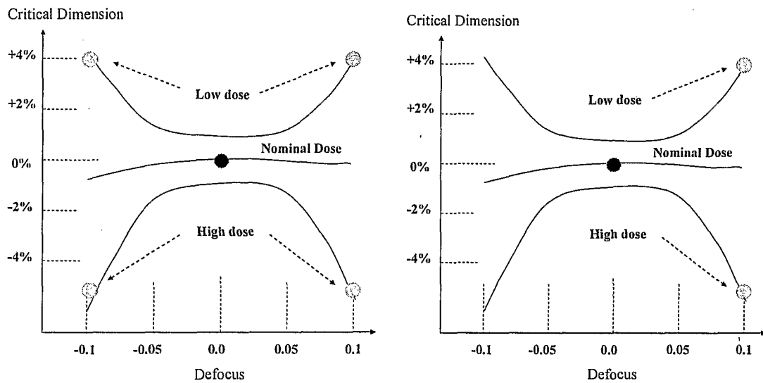
Figure 25. Effect of Exposure Dose and Defocus for a Clear field line. Indicating four process corners (left). Indicating response corners (right).
