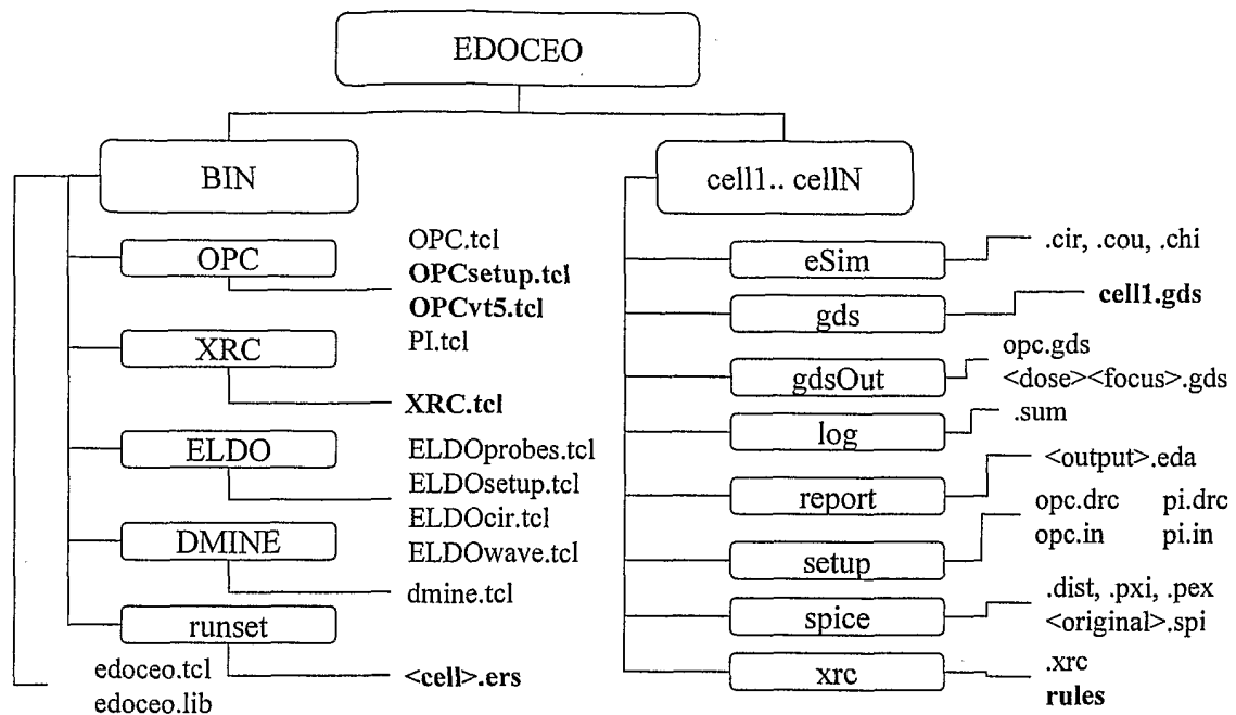
Figure 38. EDOCEO components.
