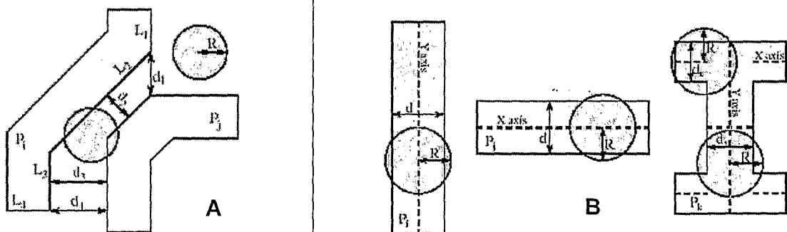
Figure 6. Critical area calculation depicting short (A) and open (B) defects.
