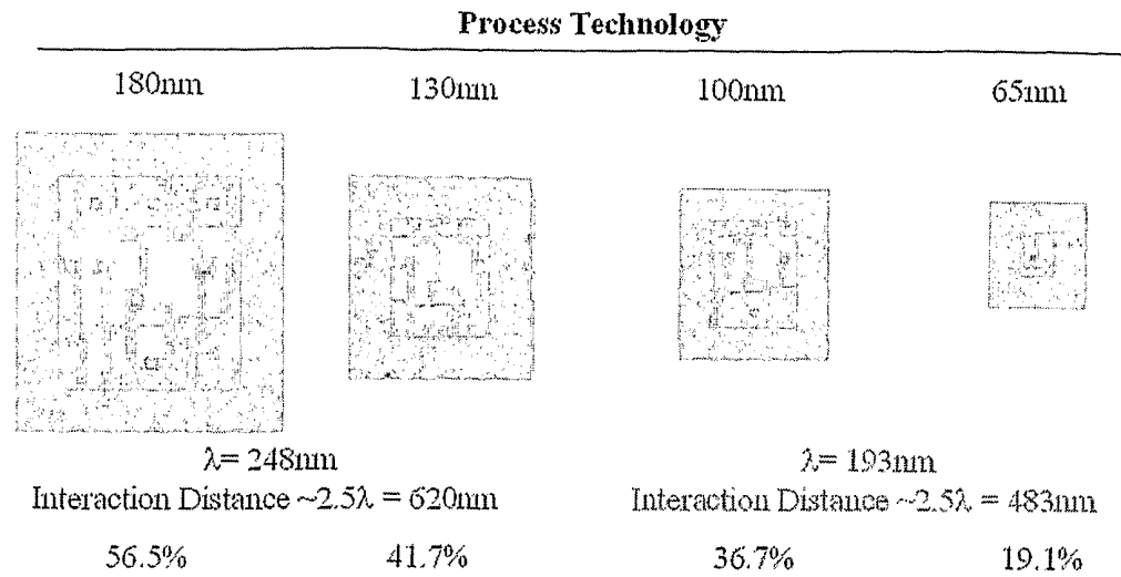
Figure 20. Placement-independent areas for multiple process nodes.
