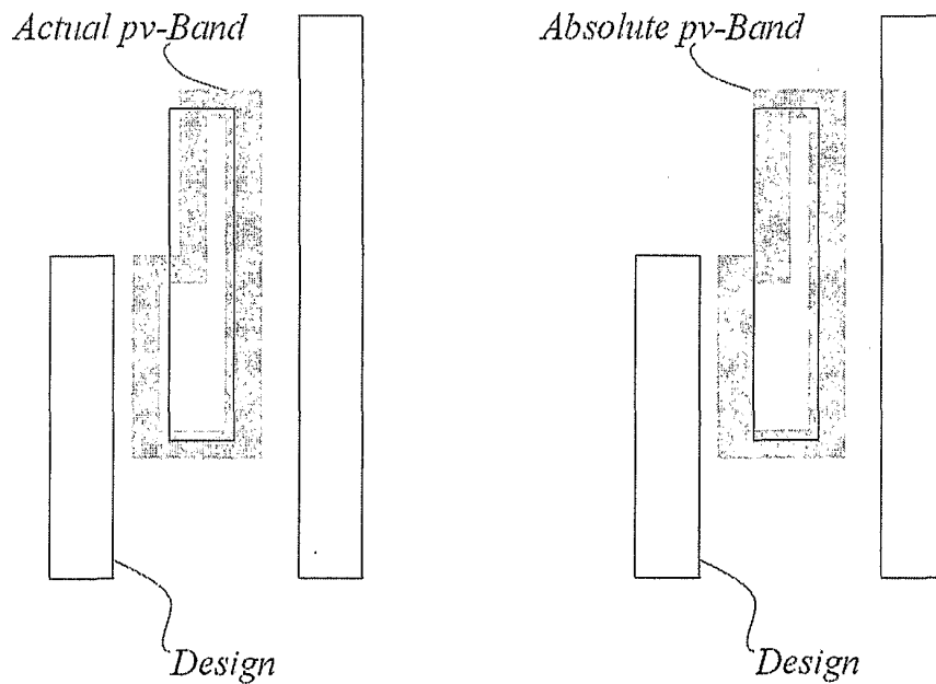
Figure 13. Actual Vs Relative pv-Bands.
