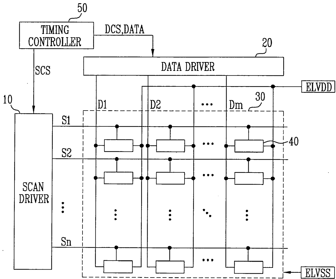
FIG. 1 (RELATED ART)
