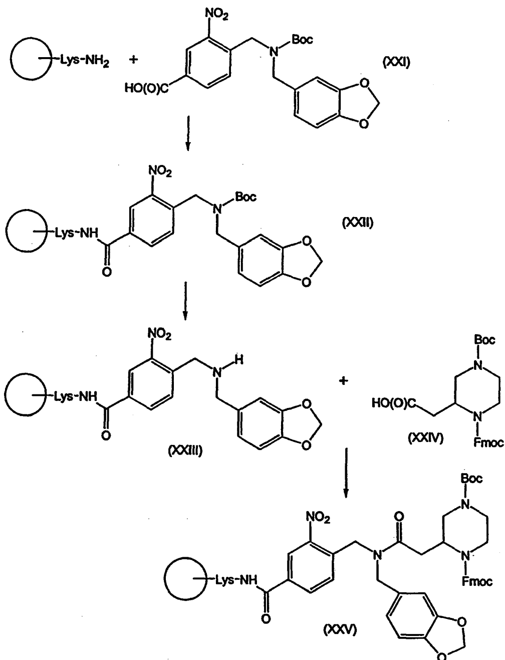
Reaction Scheme 7
