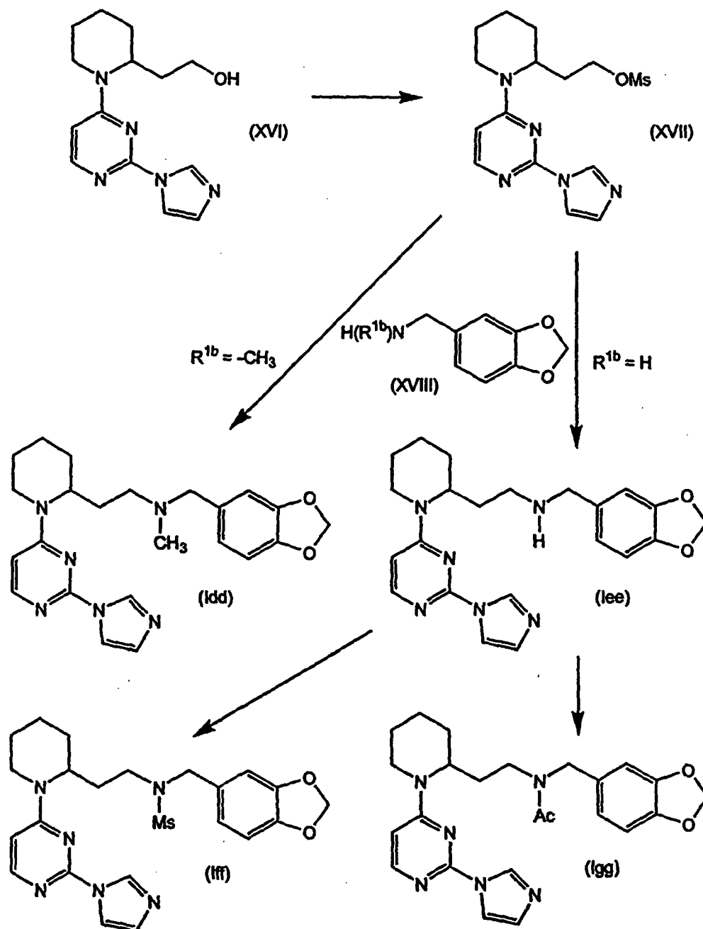
Reaction Scheme 5
