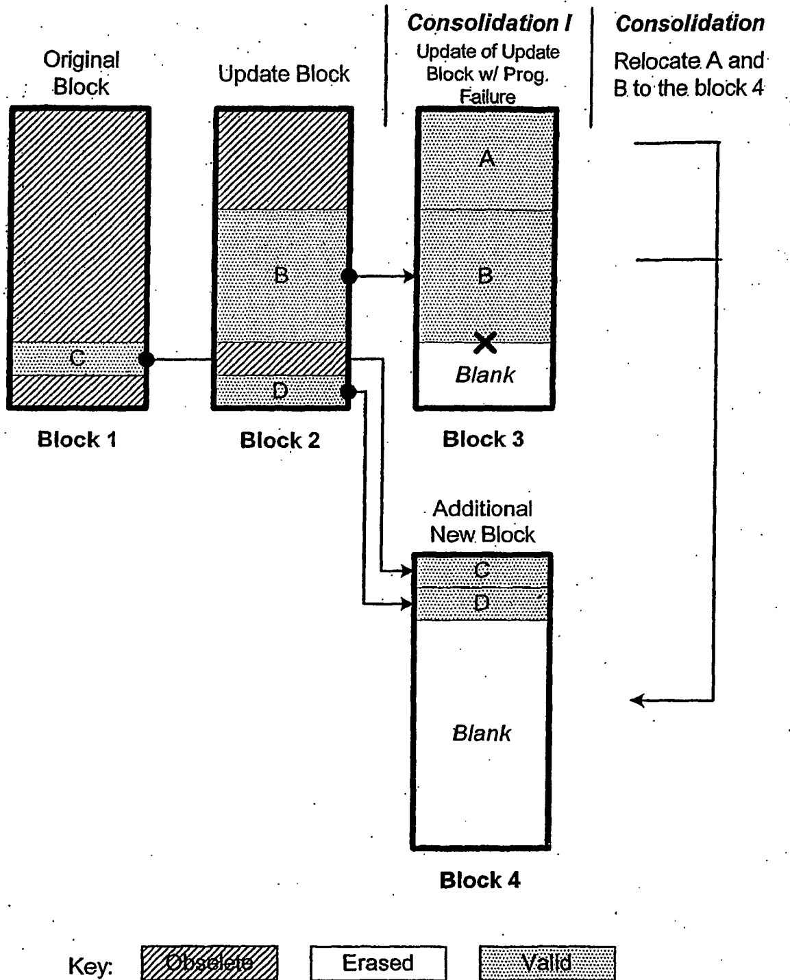
Consolidation of Update of Update Block Failure Handling (Phase I and III)
