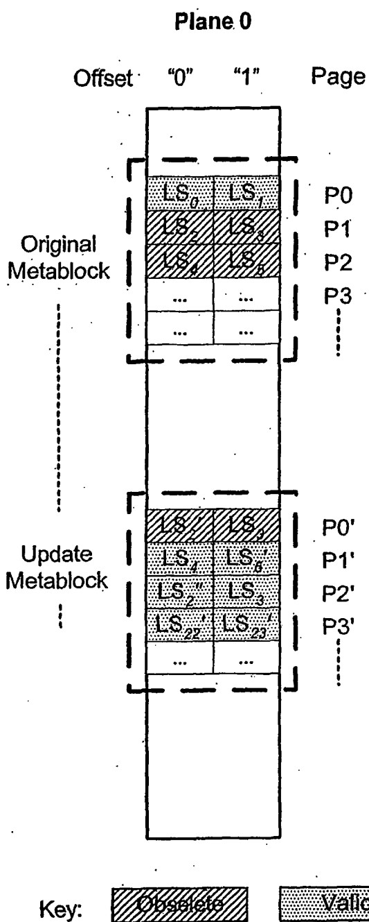
SECTOR ALIGNMENT WITHIN PAGE Exampe
