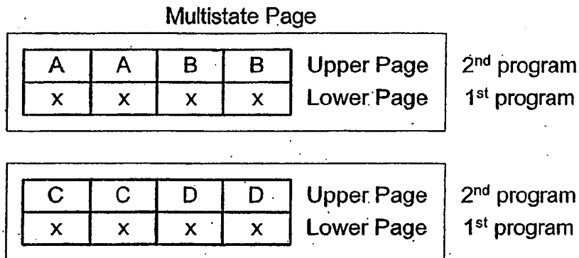
Duplicate Sectors in Upper Page Only
