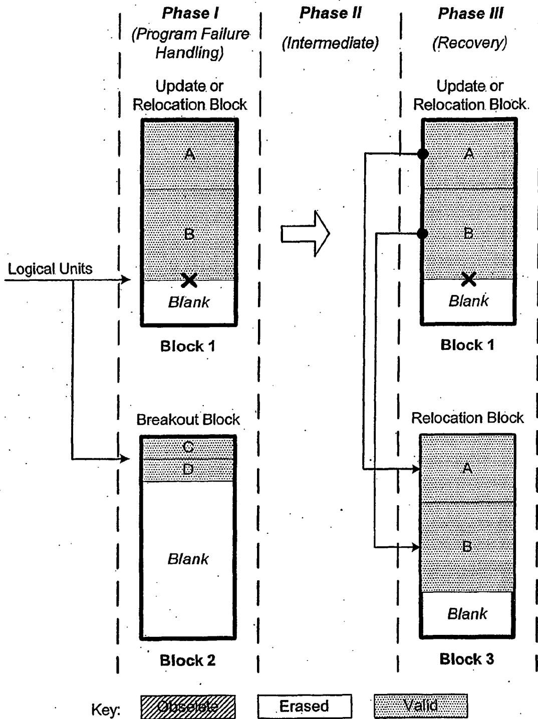
Program Failure Handling (Case 1: Block 3 = New)
