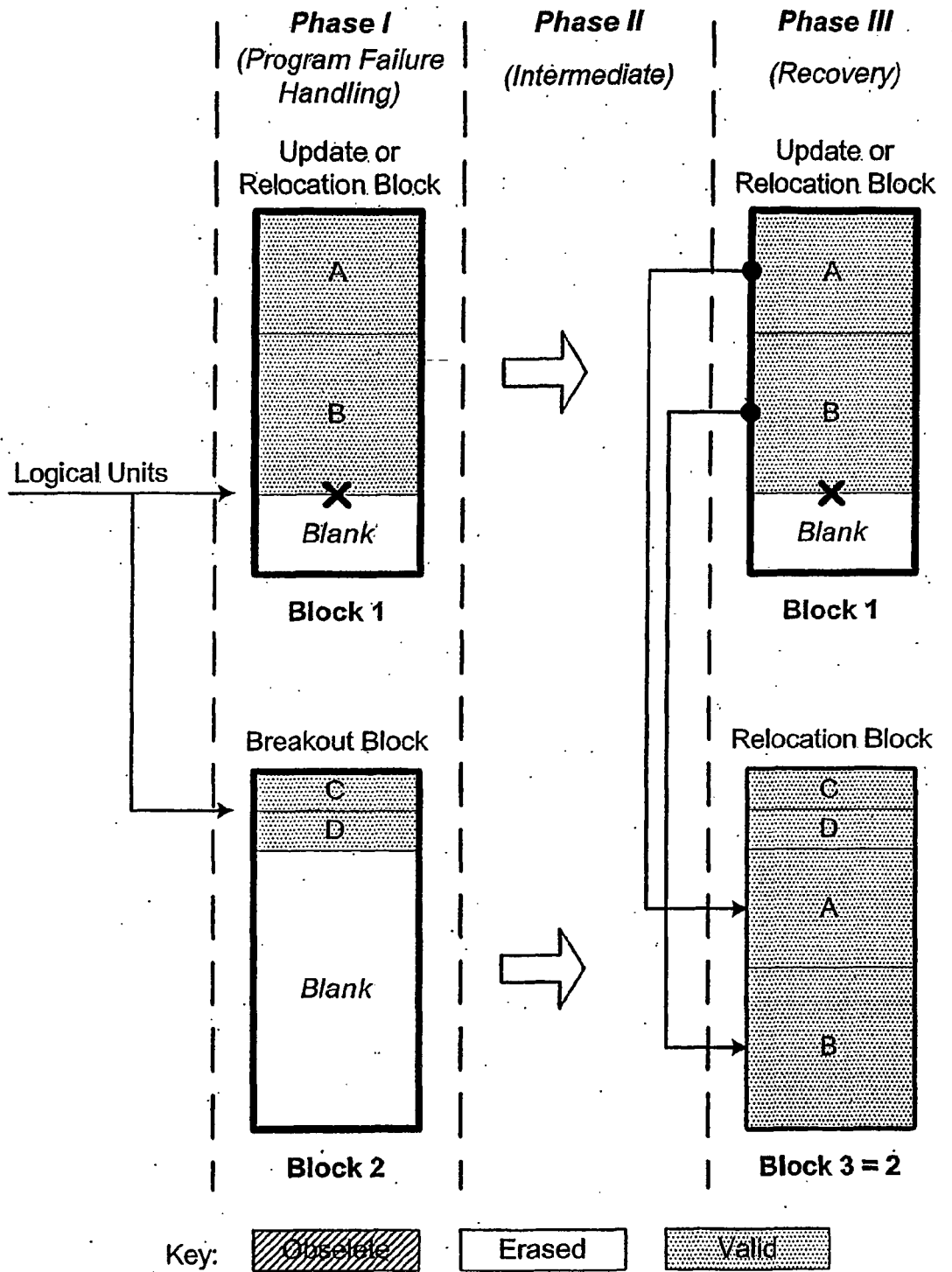
Program Failure Handling (Case 2: Block 3 = Block 2)
