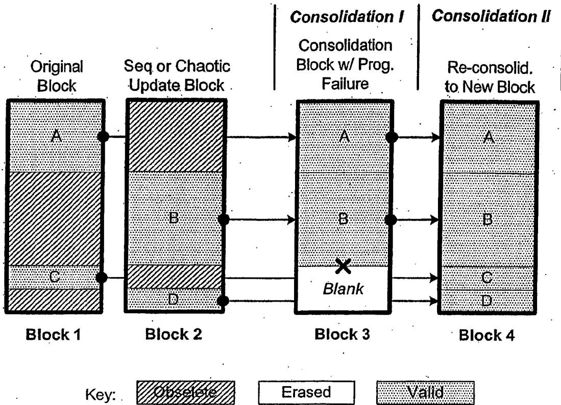
Consolidation Failure Handling by Re-consolidation
