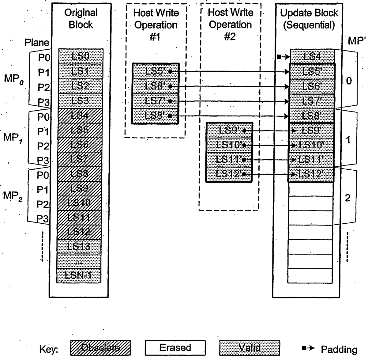
PLANE-ALIGNED SEQUENTIAL UPDATE Example
