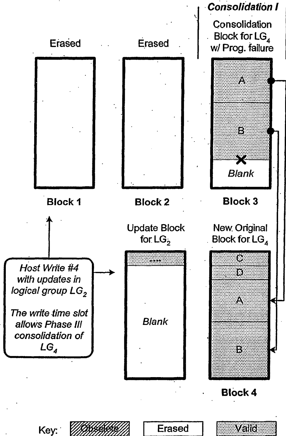
Consolidation Failure Handling (Phase III) (Case 1: No additional updates on Breakout Block)
