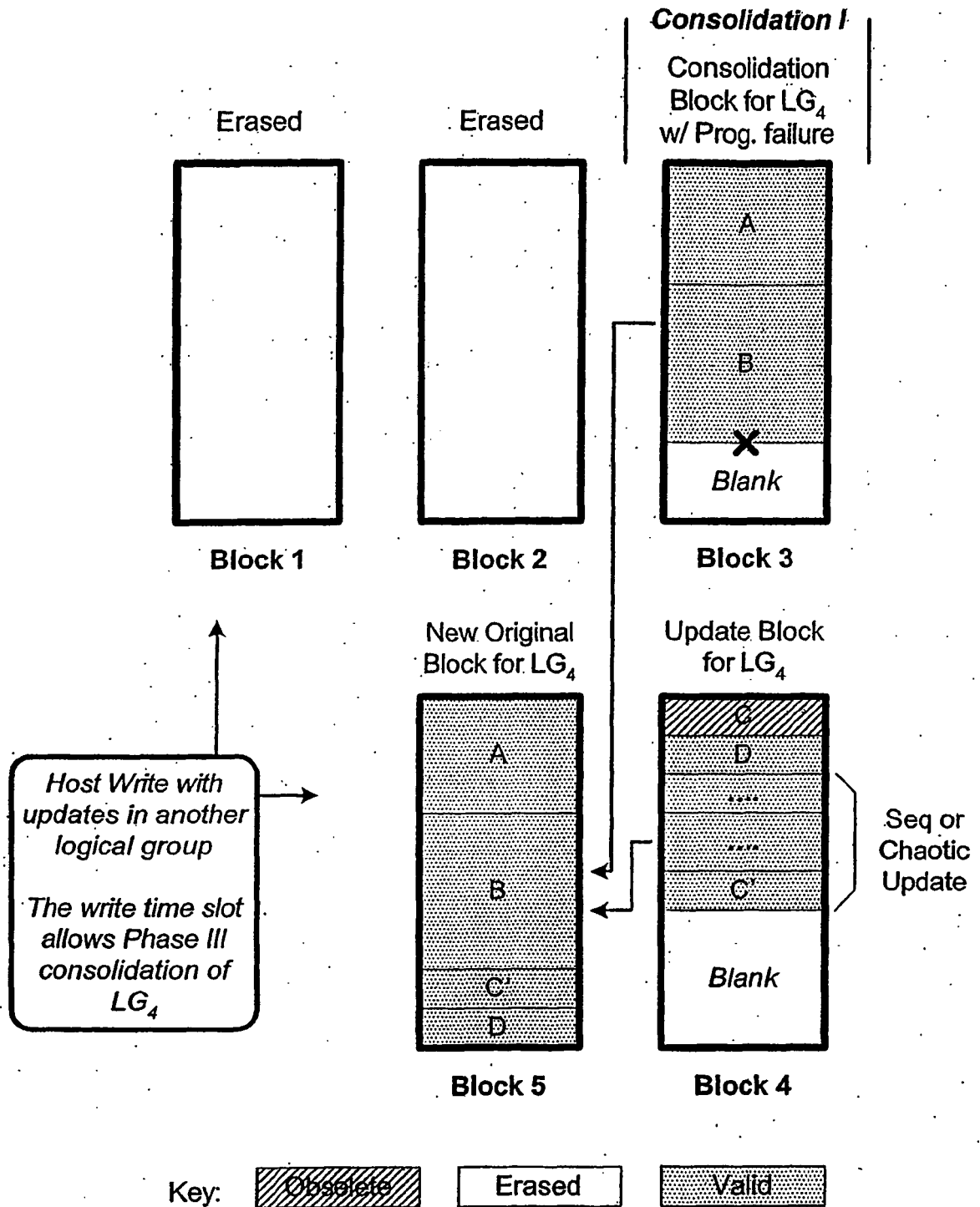
Consolidation Failure Handling (Phase III) (Case 2: Additional updates on Breakout Block)
