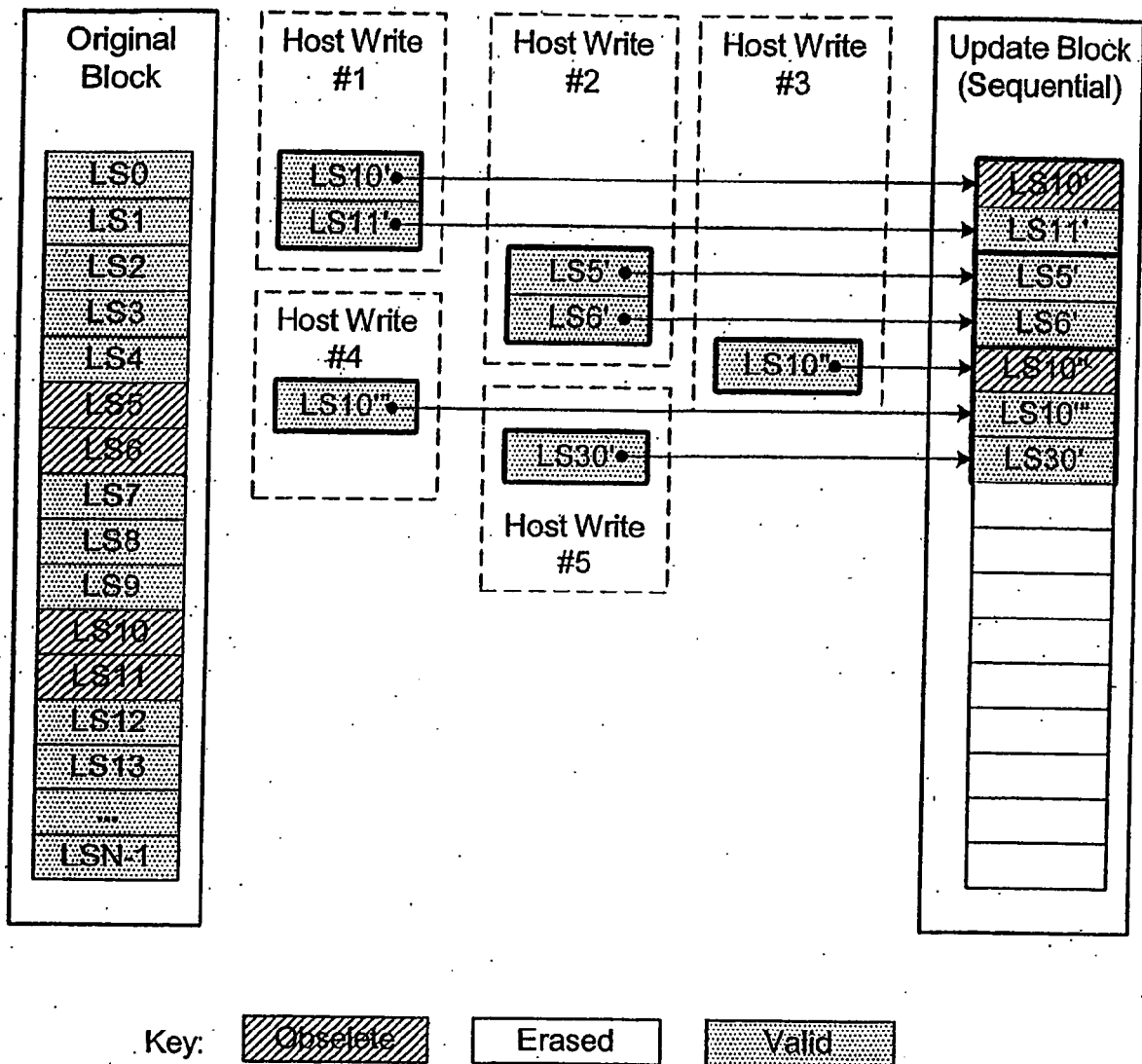
CHAOTIC UPDATE (NONSEQUENTIAL) Example
