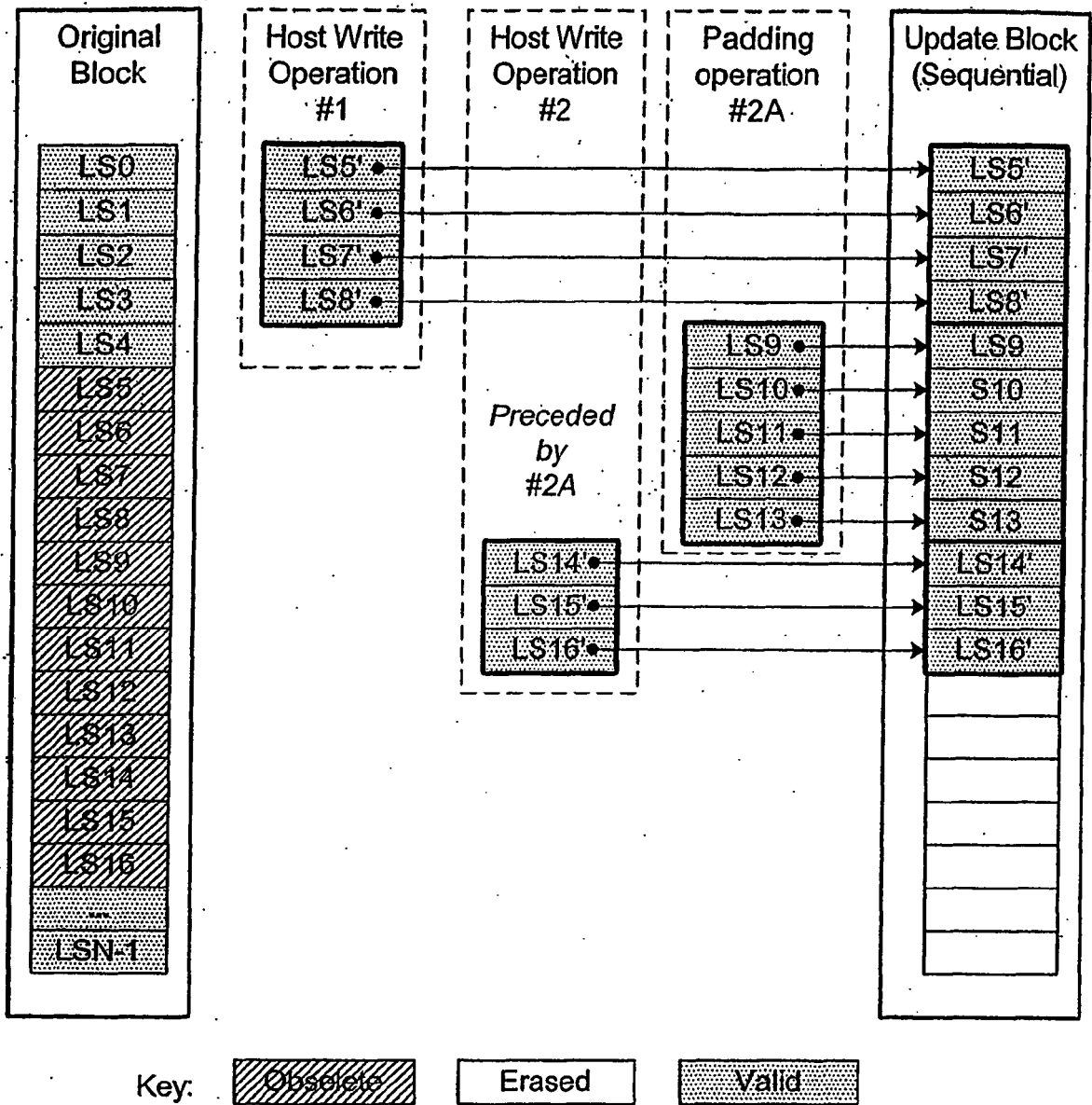
FORCED SEQUENTIAL UPDATE Example
