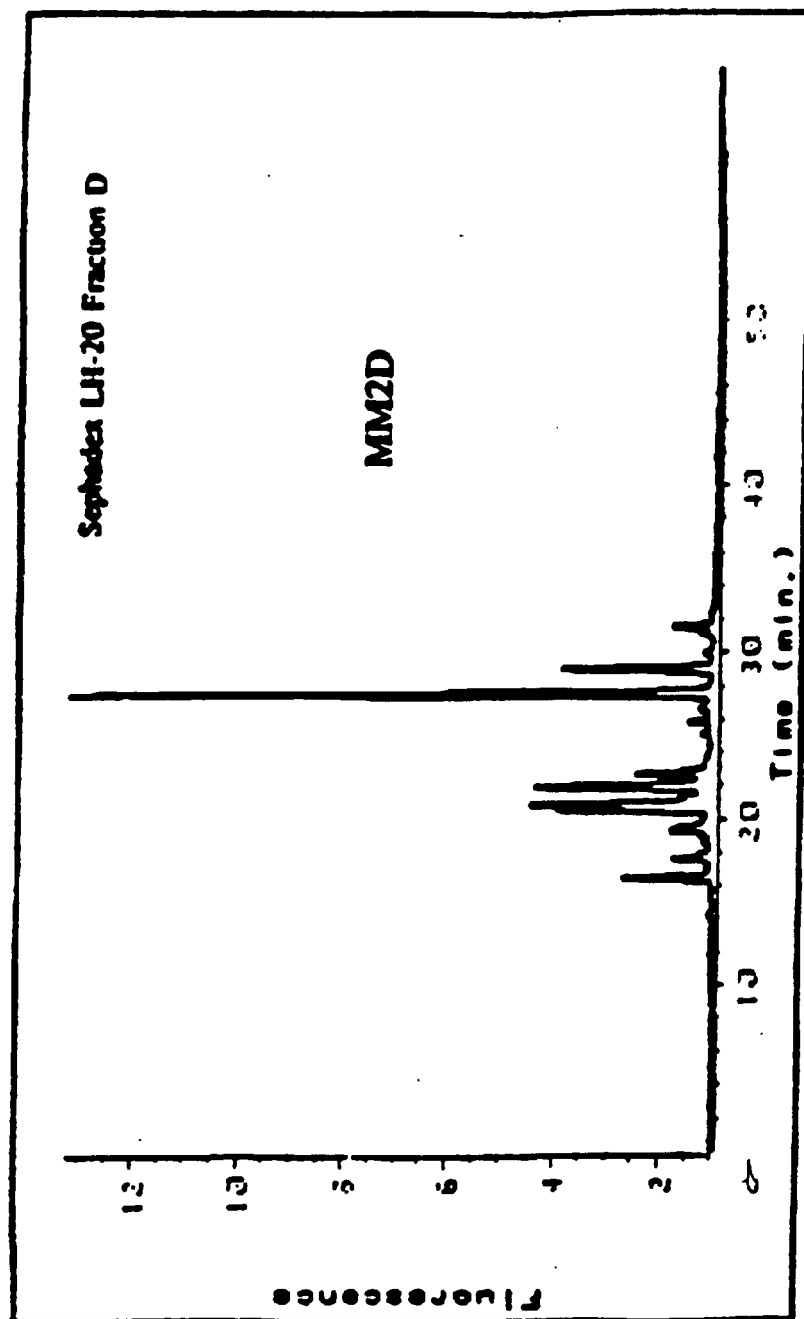
Figure 4D Representative HPLC Traces of Procyanidin Fractions
