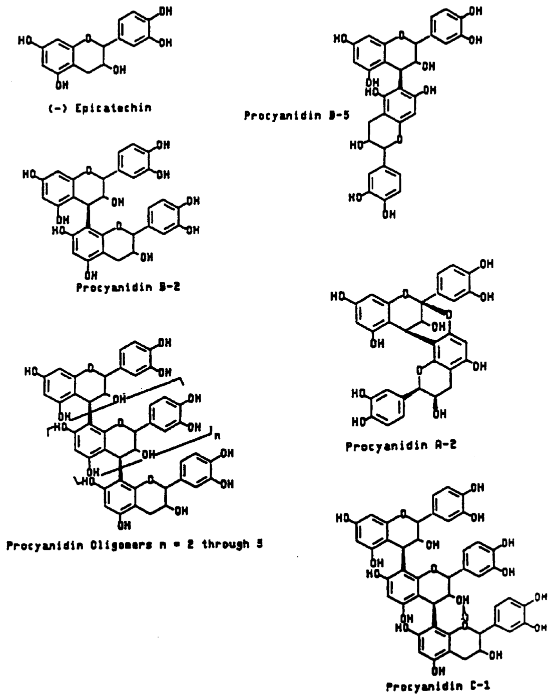
Figure 3: Representative Structures of Cocoa Procyanidins
