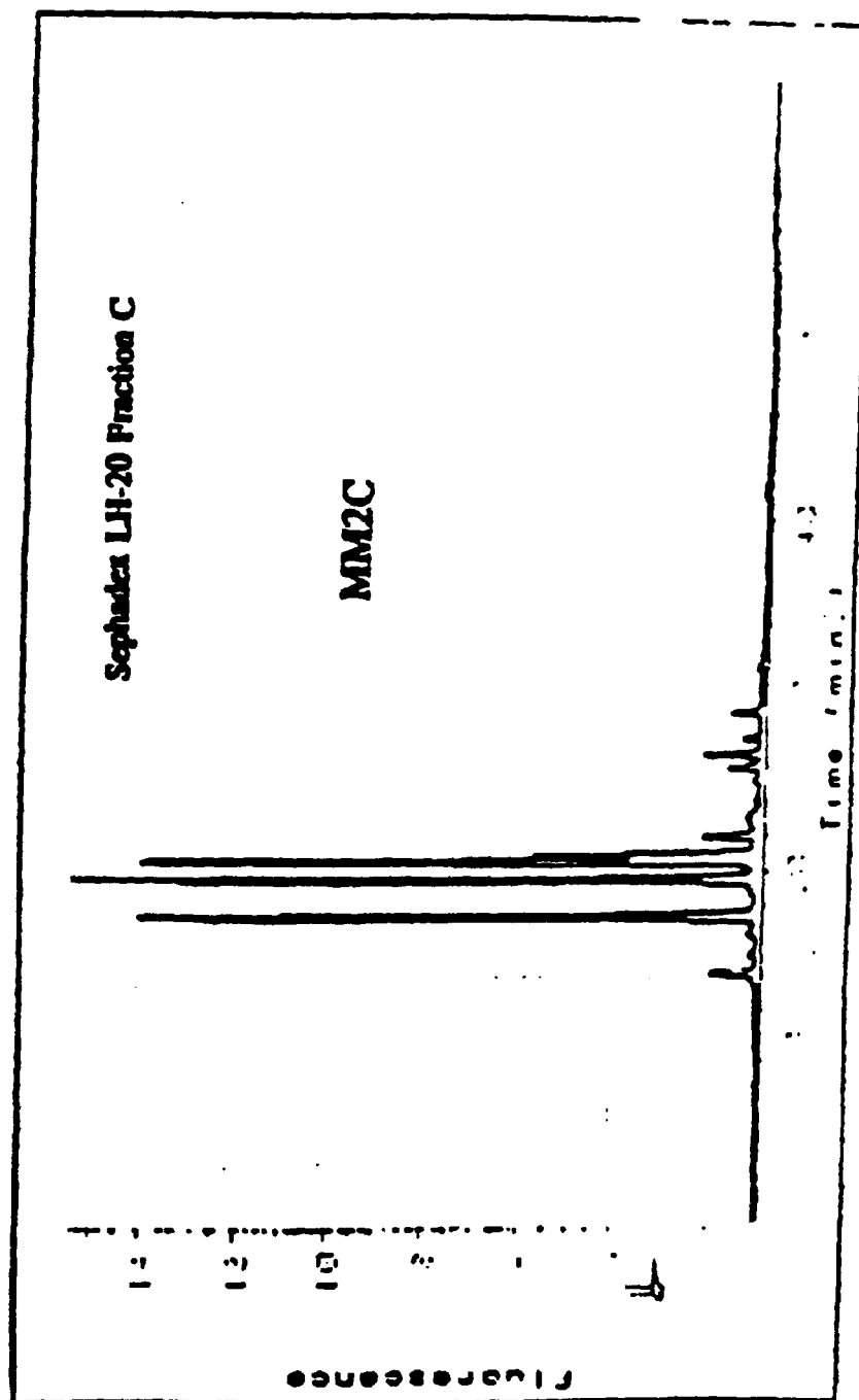
Figure 4C Representative HPLC Traces of Procyanidin Fractions
