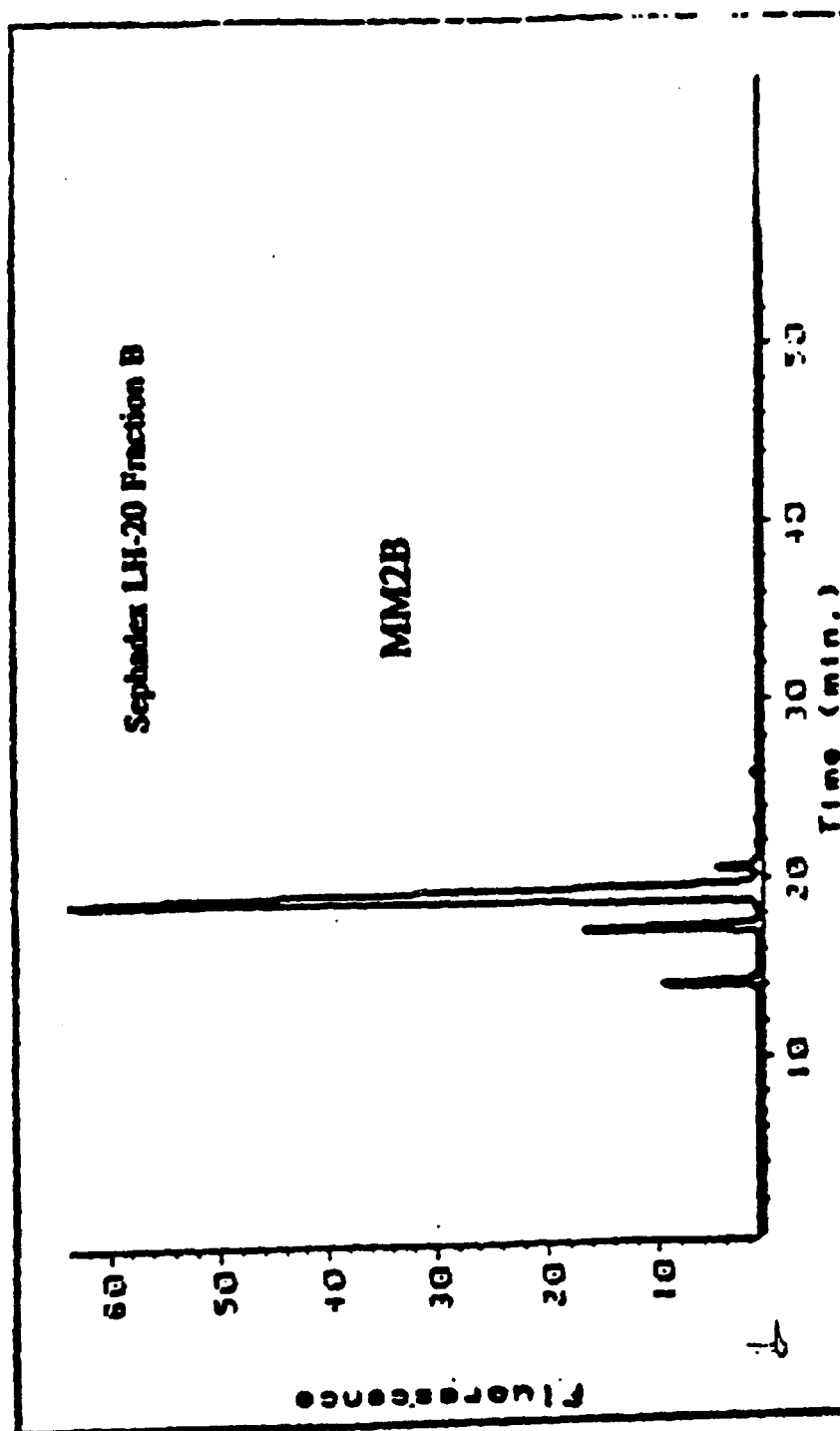
Figure 4B Representative HPLC Traces of Procyanidin Fractions
