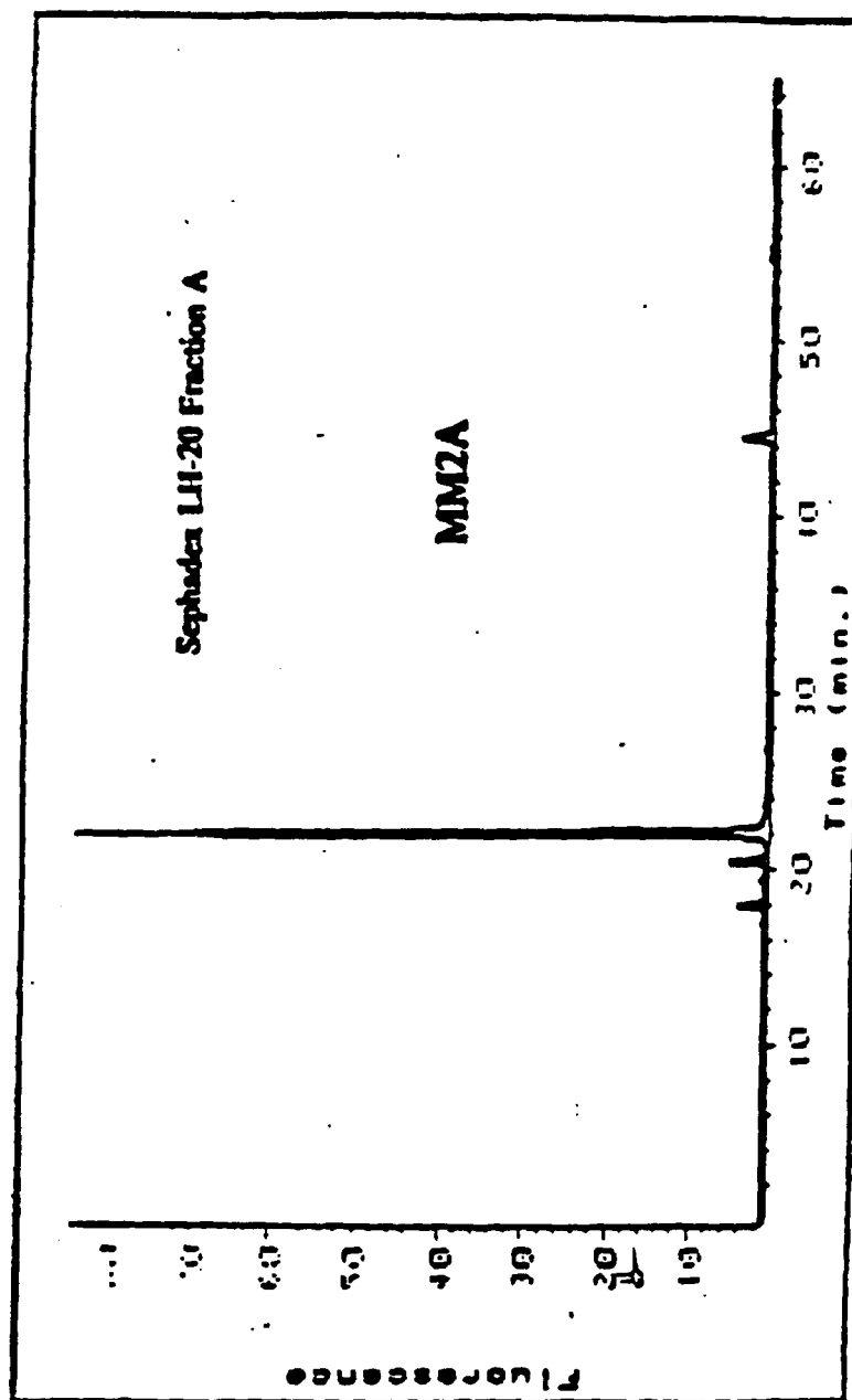
Figure 4A Representative HPLC Traces of Procyanidin Fractions
