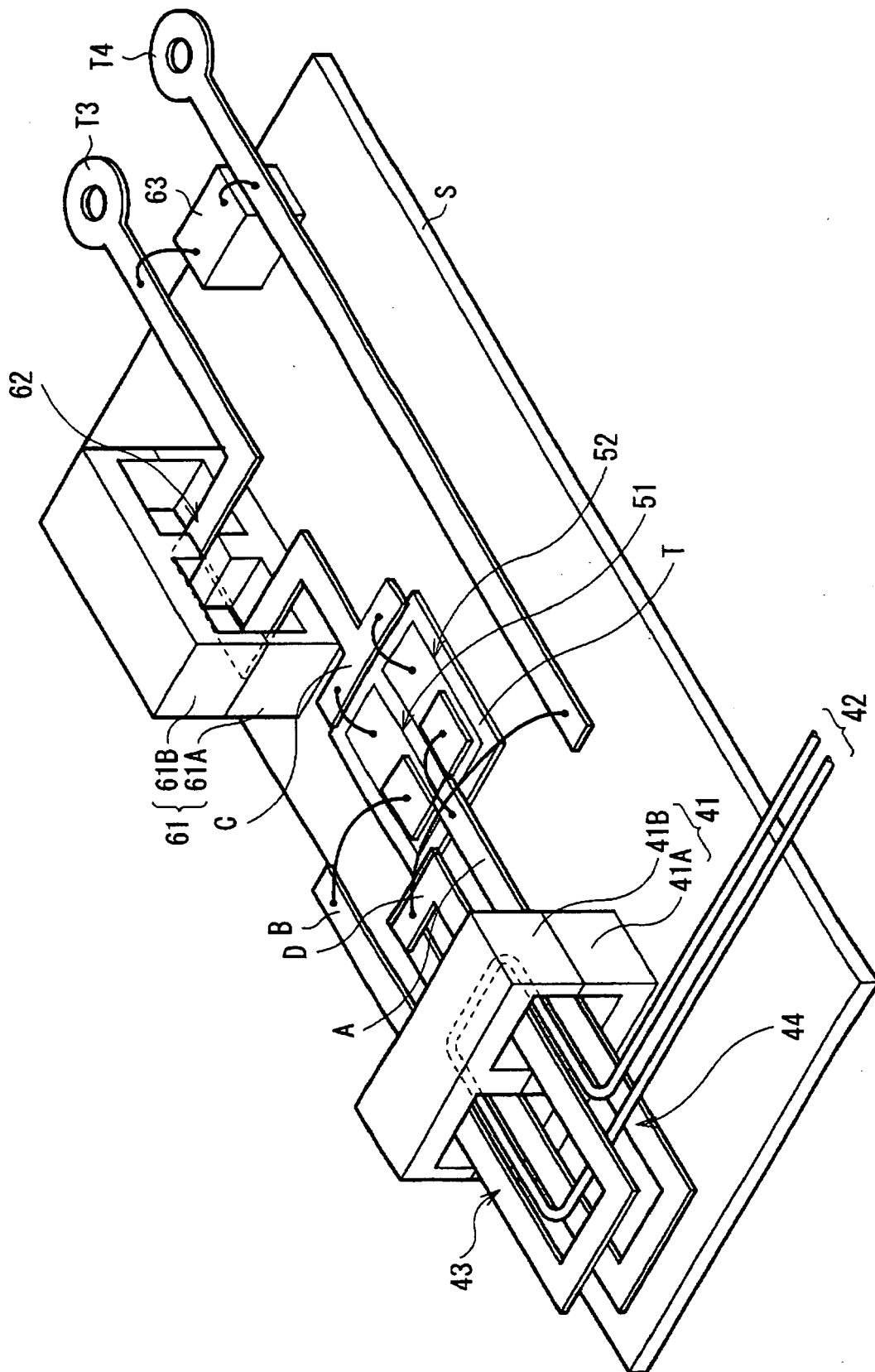
FIG. 4 RELATED ART
