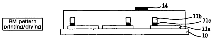
Fig.3F (Related Art)
