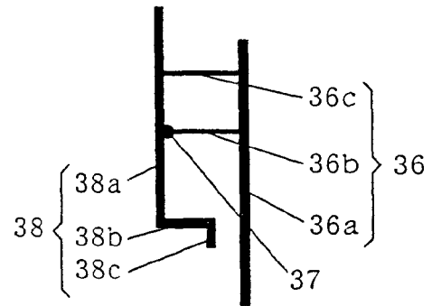
CROSS-SECTIONAL SIDE VIEW FROM ANTENNA-HOUSING BASE PLATE 38
