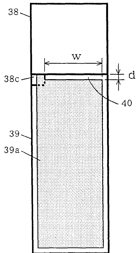
FRONT VIEW OF ANTENNA-HOUSING BASE PLATE 38 AND CIRCUIT-HOUSING BASE PLATE 39 CONNECTED TO EACH OTHER
